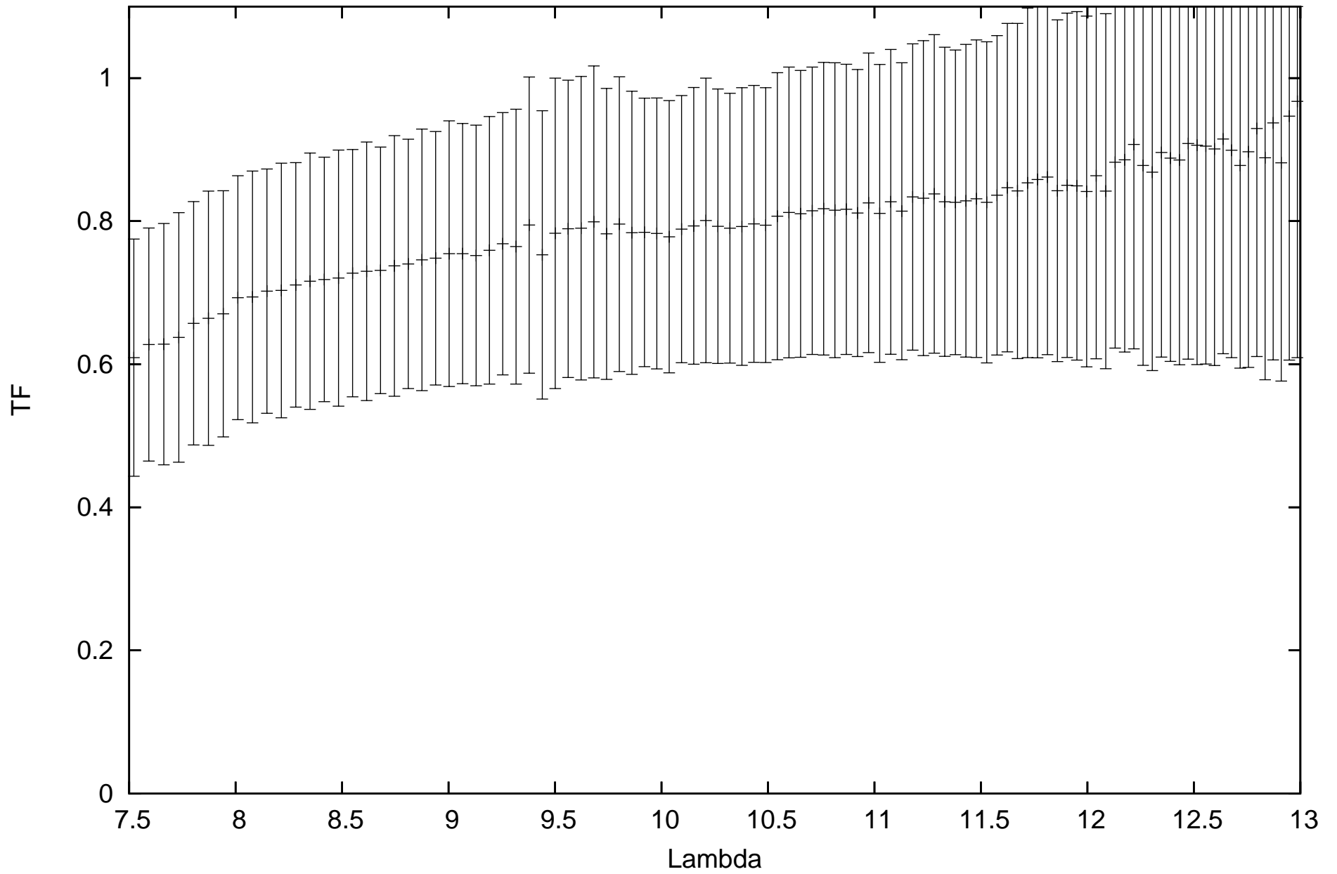
calHD167618_flux-1.82_diam11.66_r.MIDI.2010-08-21T03_42_03.000_H011
