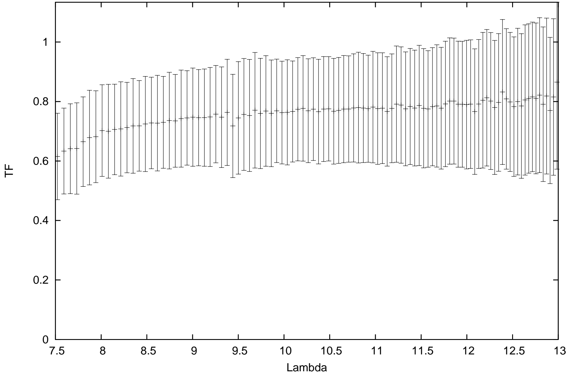
calHD167618_flux-1.82_diam11.66_r.MIDI.2010-08-21T03_16_35.000_H011
