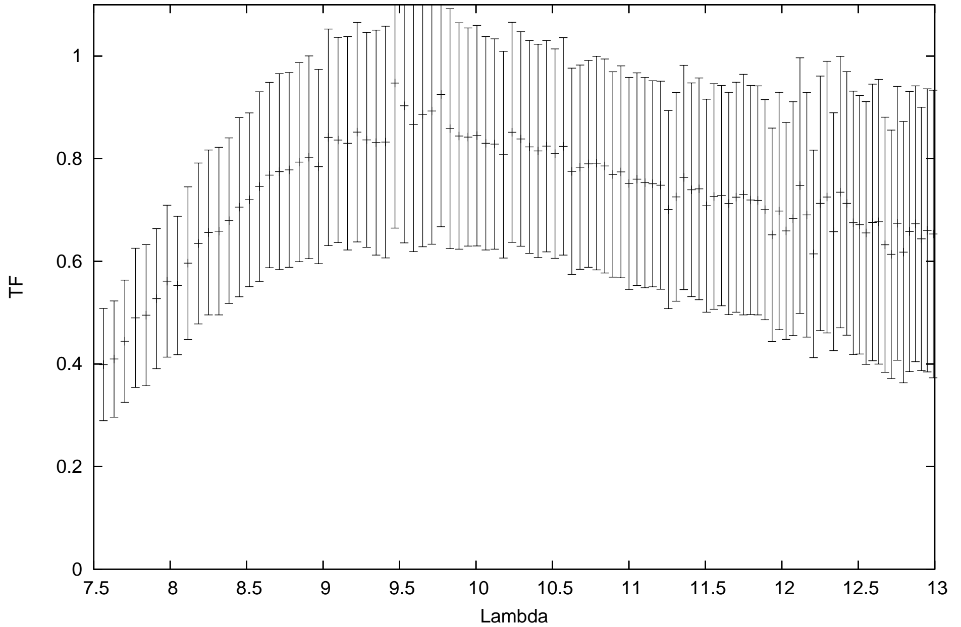
calHD167618_flux-1.82_diam11.66_r.MIDI.2010-08-21T02_28_24.138_H011
