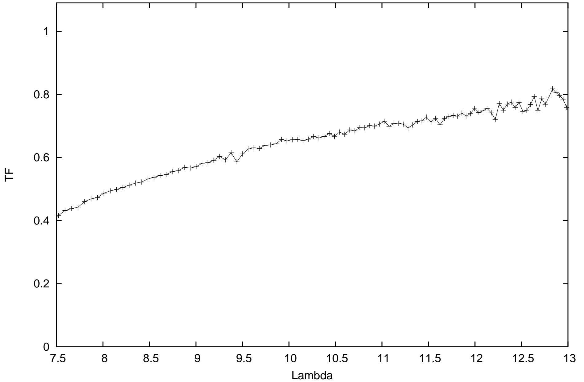
calHD133216_flux-1.76_diam11.15_r.MIDI.2010-07-10T01_07_21.000_D0I1
