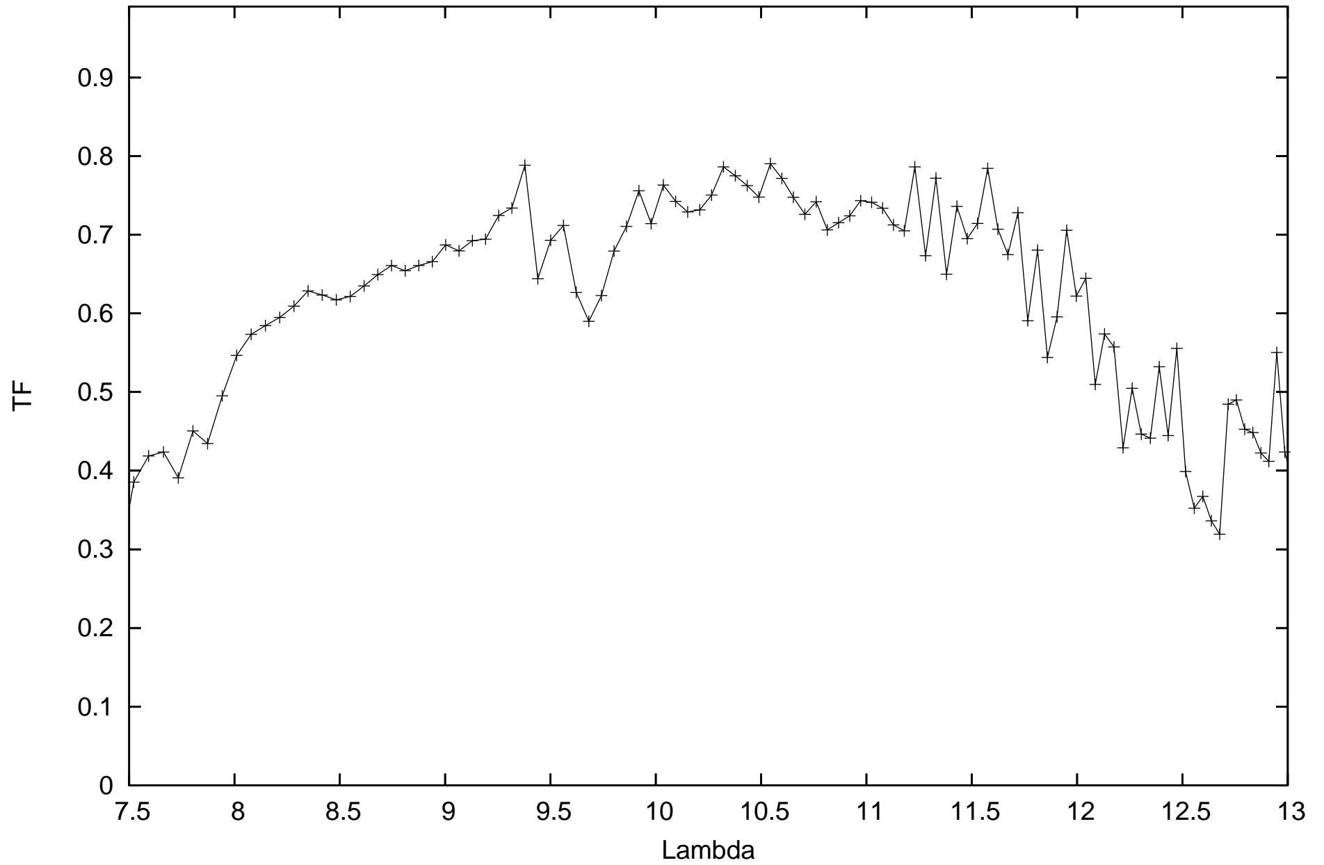
calHD187642_flux0.2_diam3.31_r.MIDI.2010-06-17T09_29_11.000_A011
