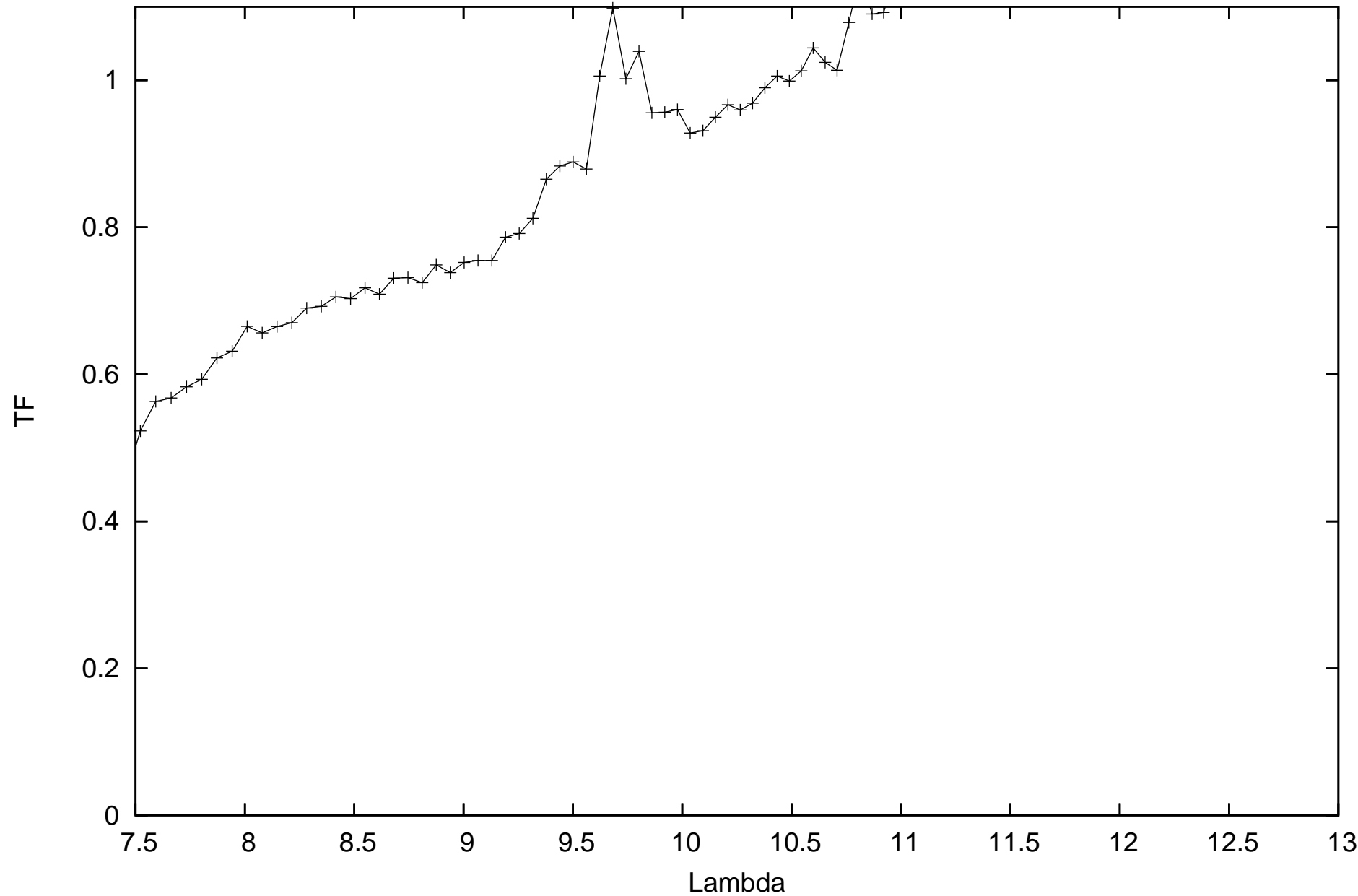
calHD169916_flux0.26_diam3.99_r.MIDI.2010-06-17T07_47_04.000_K0G1
