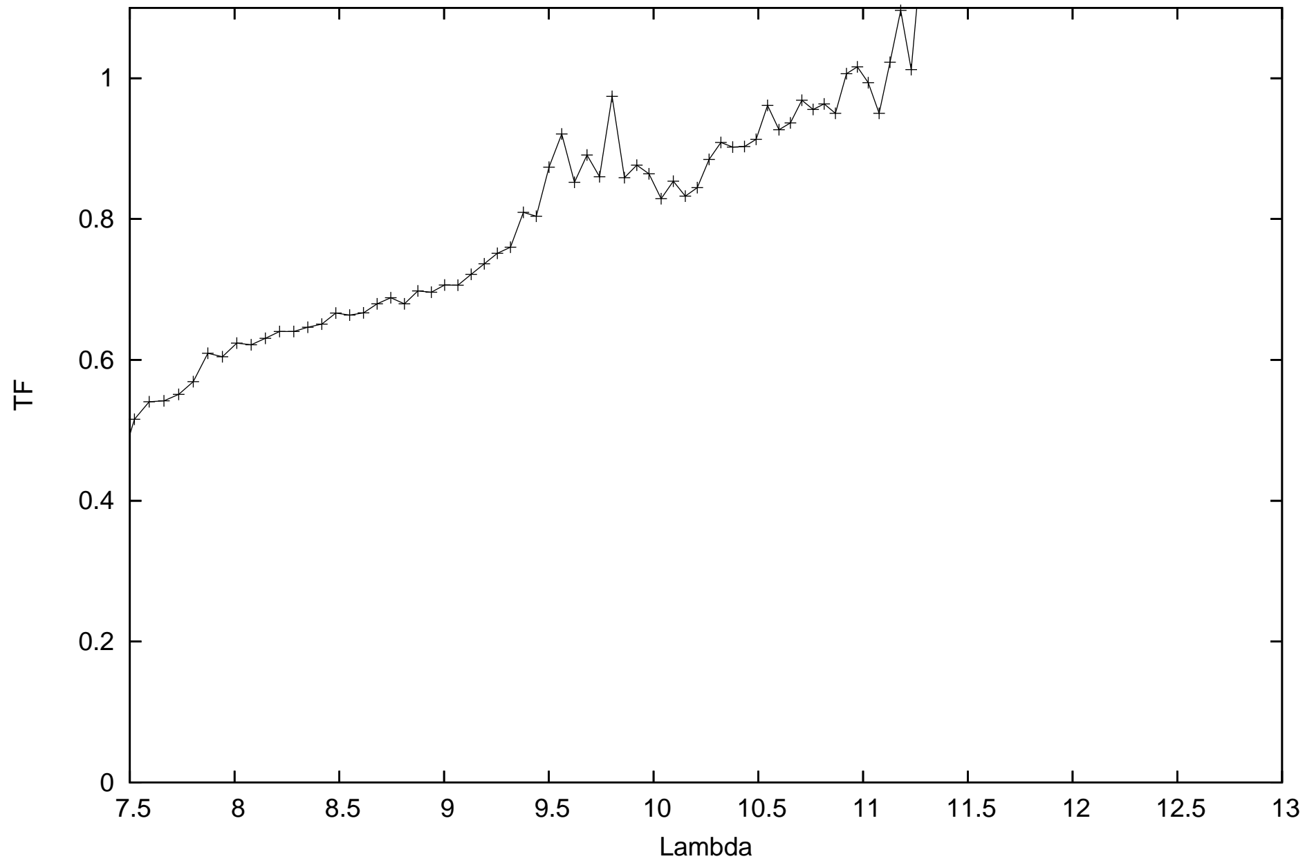
calHD169916_flux0.26_diam3.99_r.MIDI.2010-06-17T07_13_19.000_K0G1
