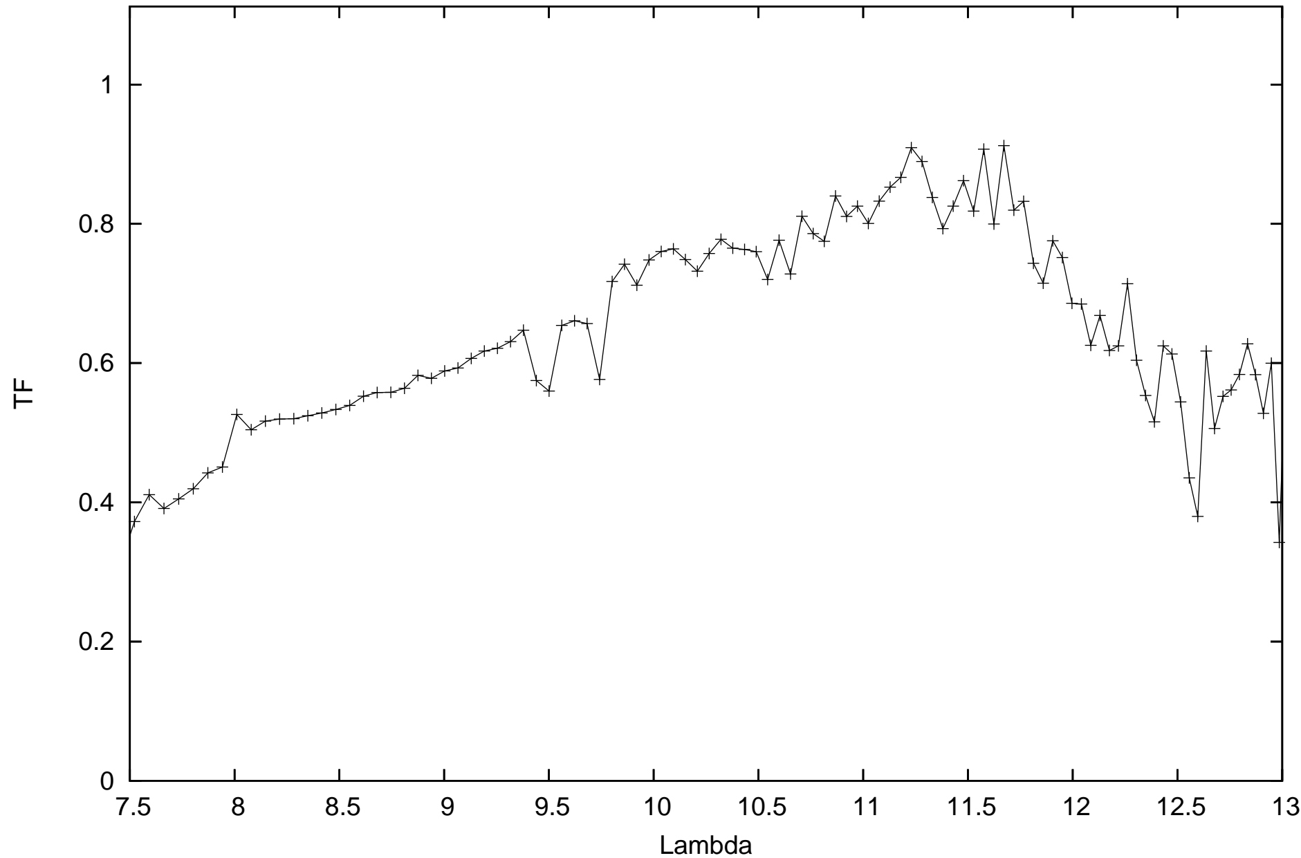
calHD152980_flux0.64_diam3.62_r.MIDI.2010-06-17T04_38_12.000_K0G1
