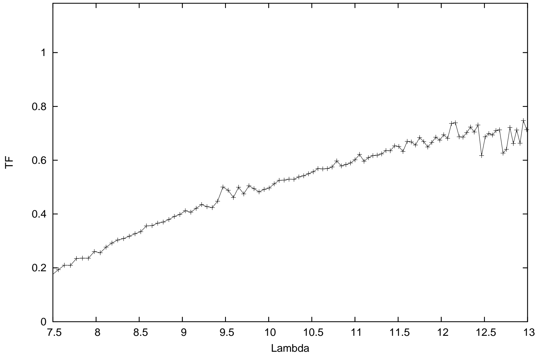
calHD133216_flux-1.76_diam11.15_r.MIDI.2010-06-17T04_07_44.138_K0G1
