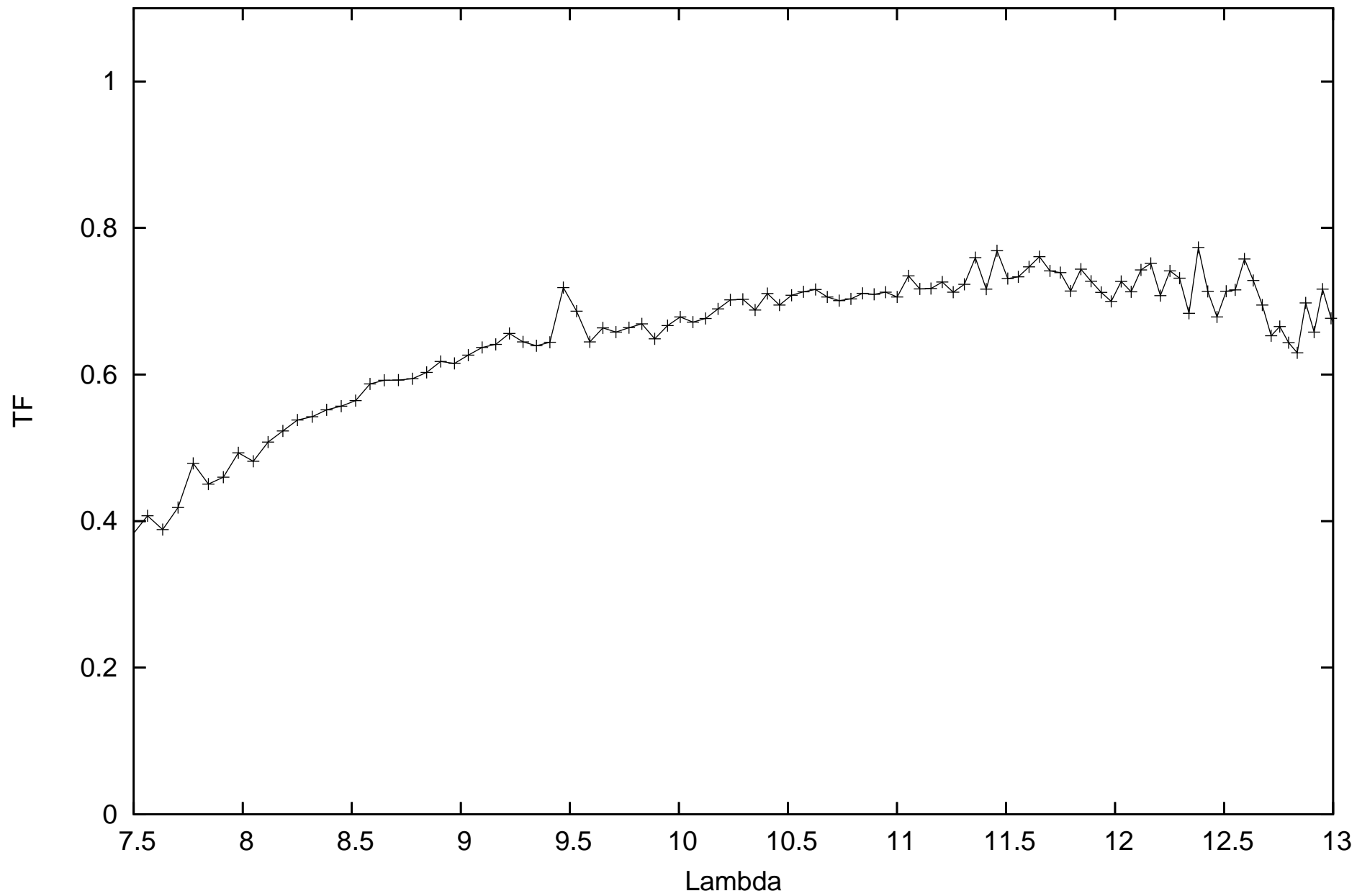
calHD167618_flux-1.82_diam11.66_r.MIDI.2010-06-12T07_22_24.180_D0H0
