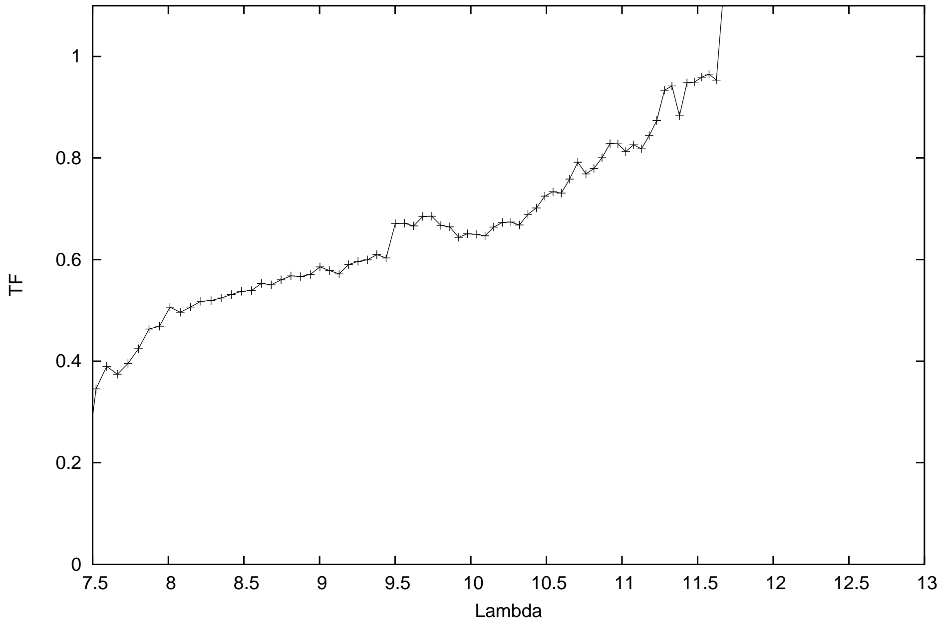
calHD168454_flux-0.48_diam5.87_r.MIDI.2010-05-21T08_32_48.000_I1E0
