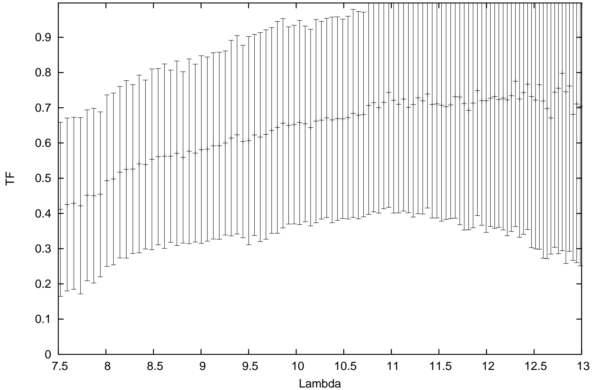
calHD168454_flux-0.48_diam5.87_r.MIDI.2010-05-21T07_39_58.000_H011
