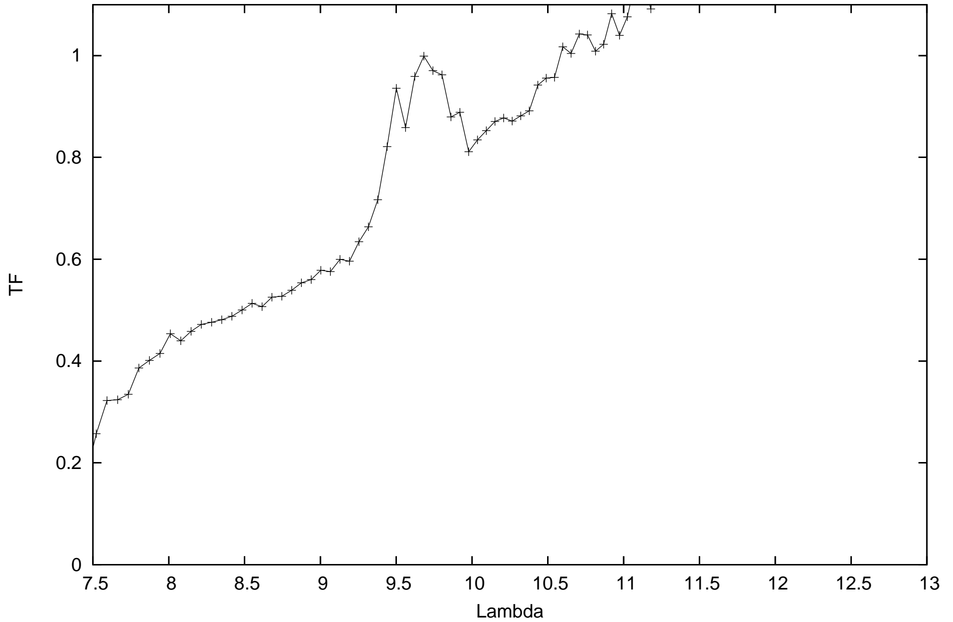
calHD152161_flux-0.26_diam6.12_r.MIDI.2010-05-21T05_44_00.000_H011
