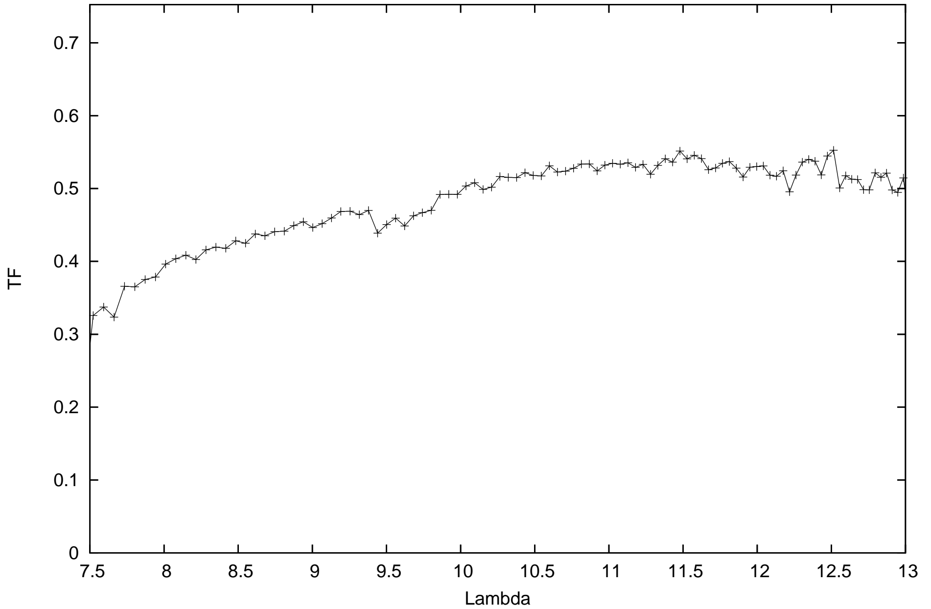
calHD081797_flux-1.49_diam9.14_r.MIDI.2010-05-21T01_42_31.000_H0E0
