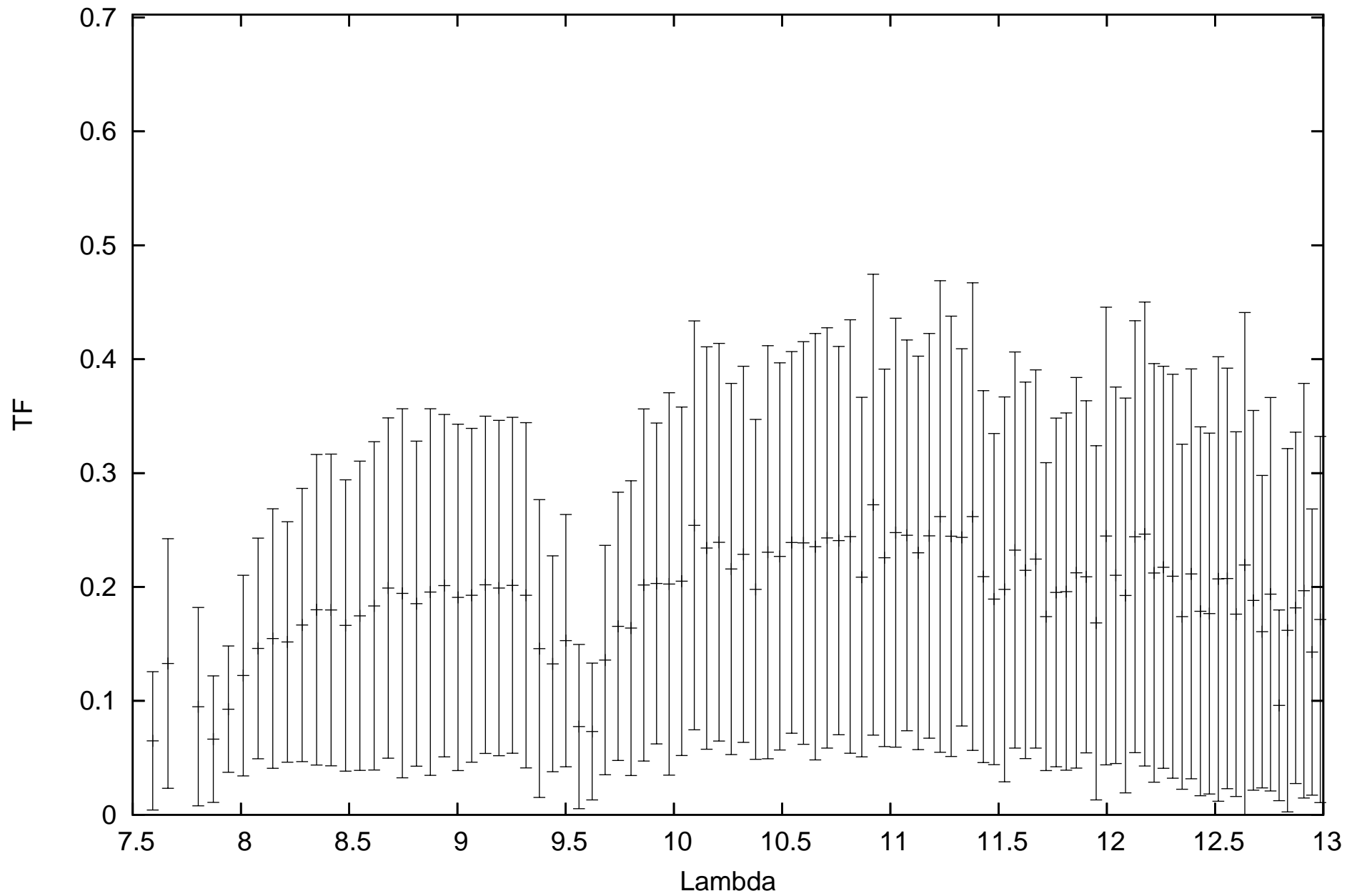
calHD107446_flux0.22_diam4.43_r.MIDI.2010-05-20T06_12_18.000_H0I1
