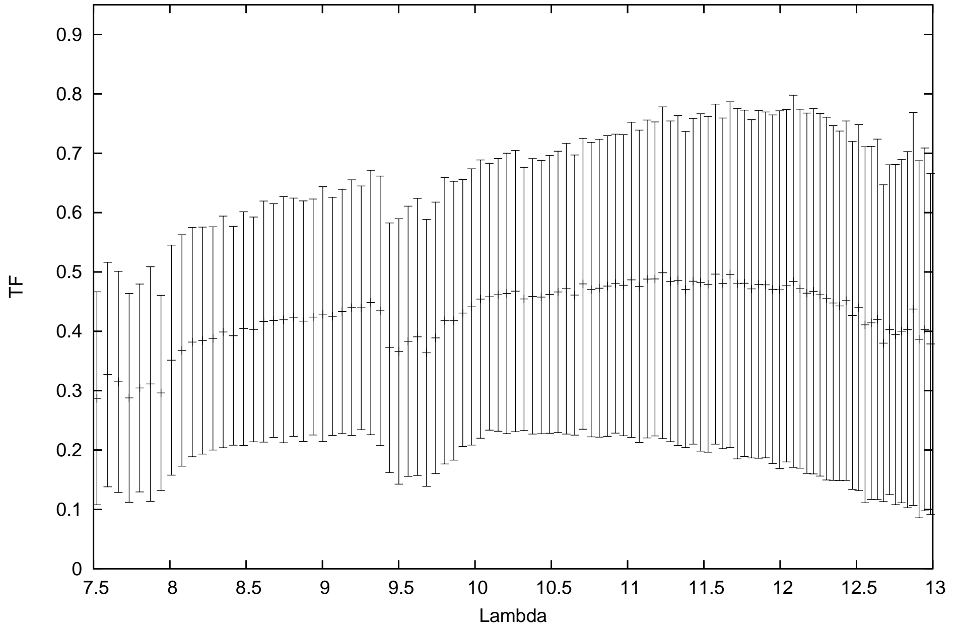
calHD152786_flux-0.79_diam6.88_r.MIDI.2010-05-05T10_35_28.000_A0G1
