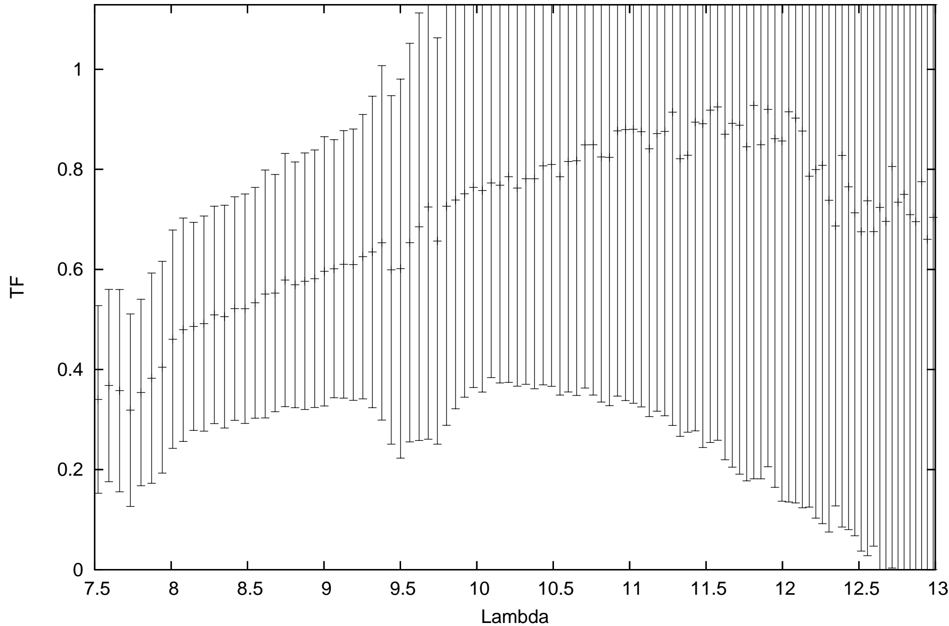
calHD107446_flux0.22_diam4.43_r.MIDI.2010-05-05T02_25_00.000_K0G1
