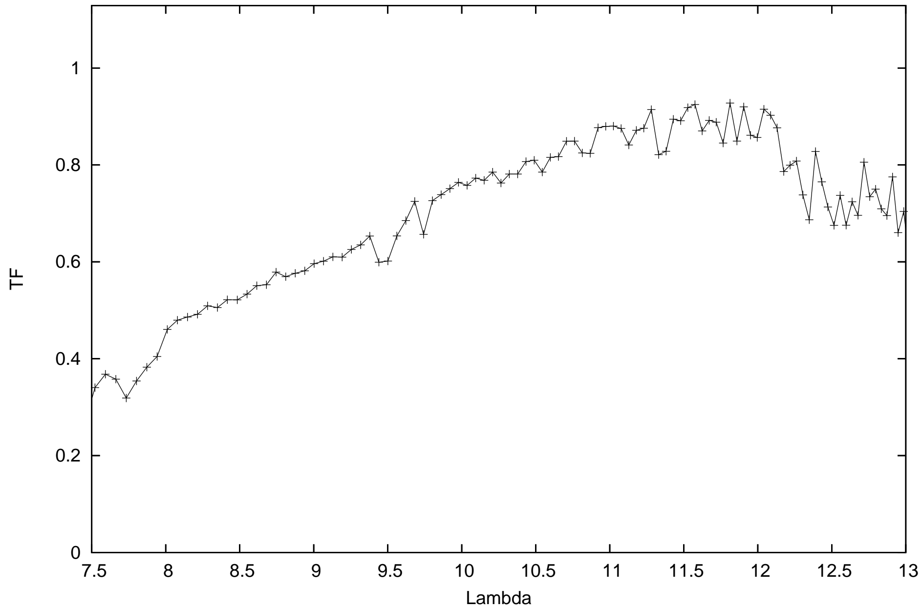
calHD107446_flux0.22_diam4.43_r.MIDI.2010-05-05T02_25_00.000_K0G1
