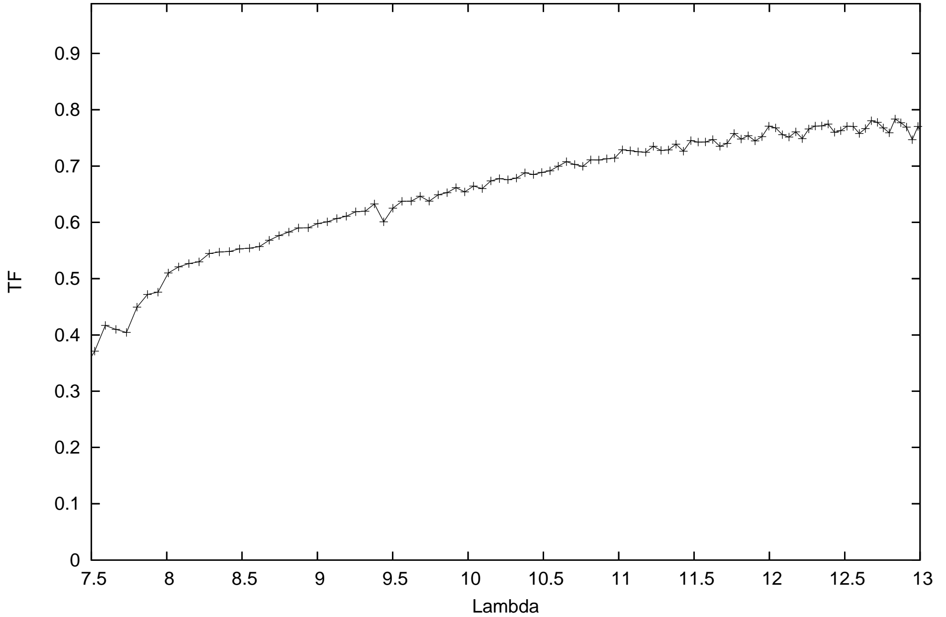
calHD082150_flux1.29_diam2.77_r.MIDI.2010-04-29T01_19_16.000_U2U4
