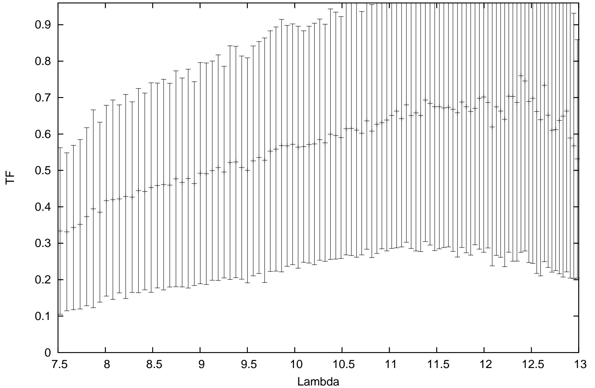
calHD152161_flux-0.26_diam6.12_r.MIDI.2010-04-19T09_27_45.000_H011
