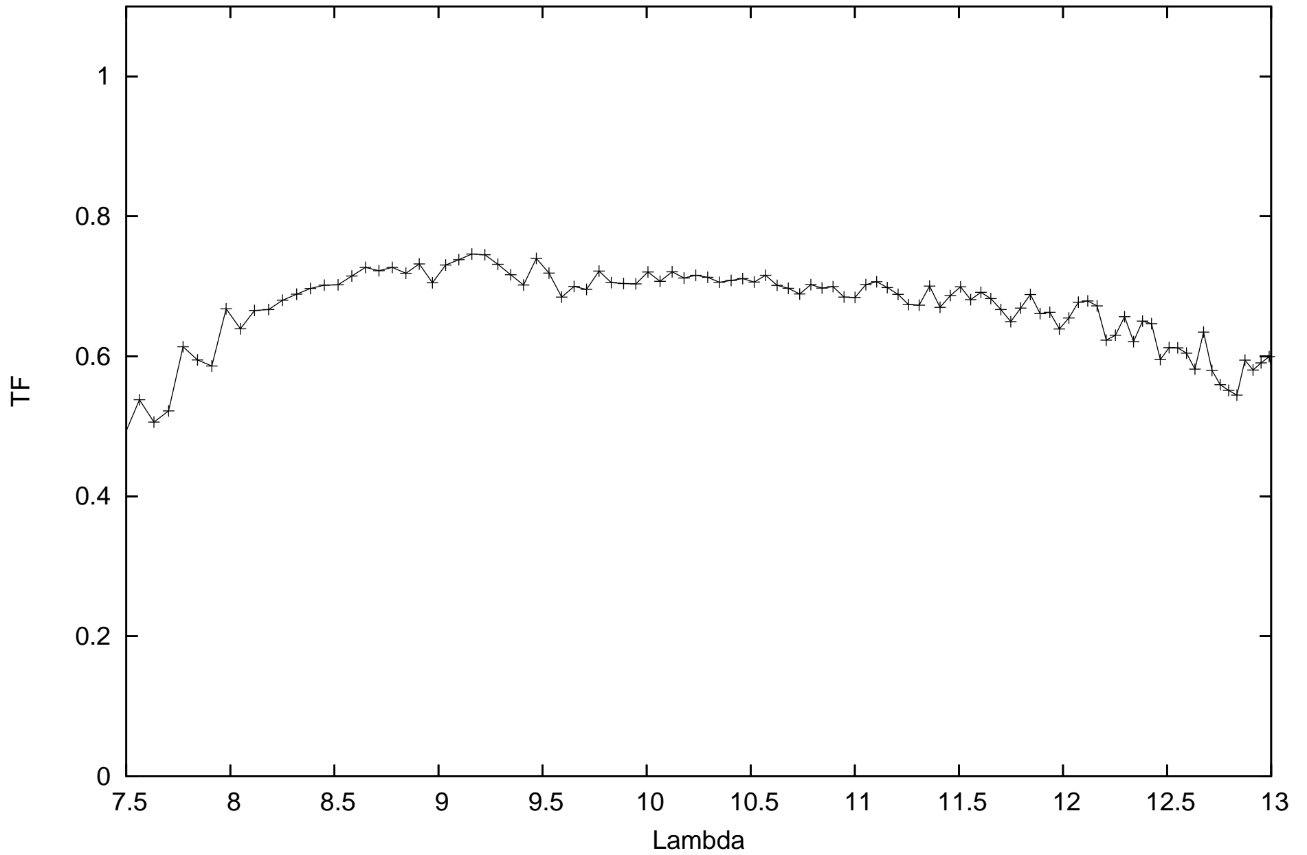
calHD081797_flux-1.49_diam9.14_r.MIDI.2010-04-13T03_36_25.138_D0H0
