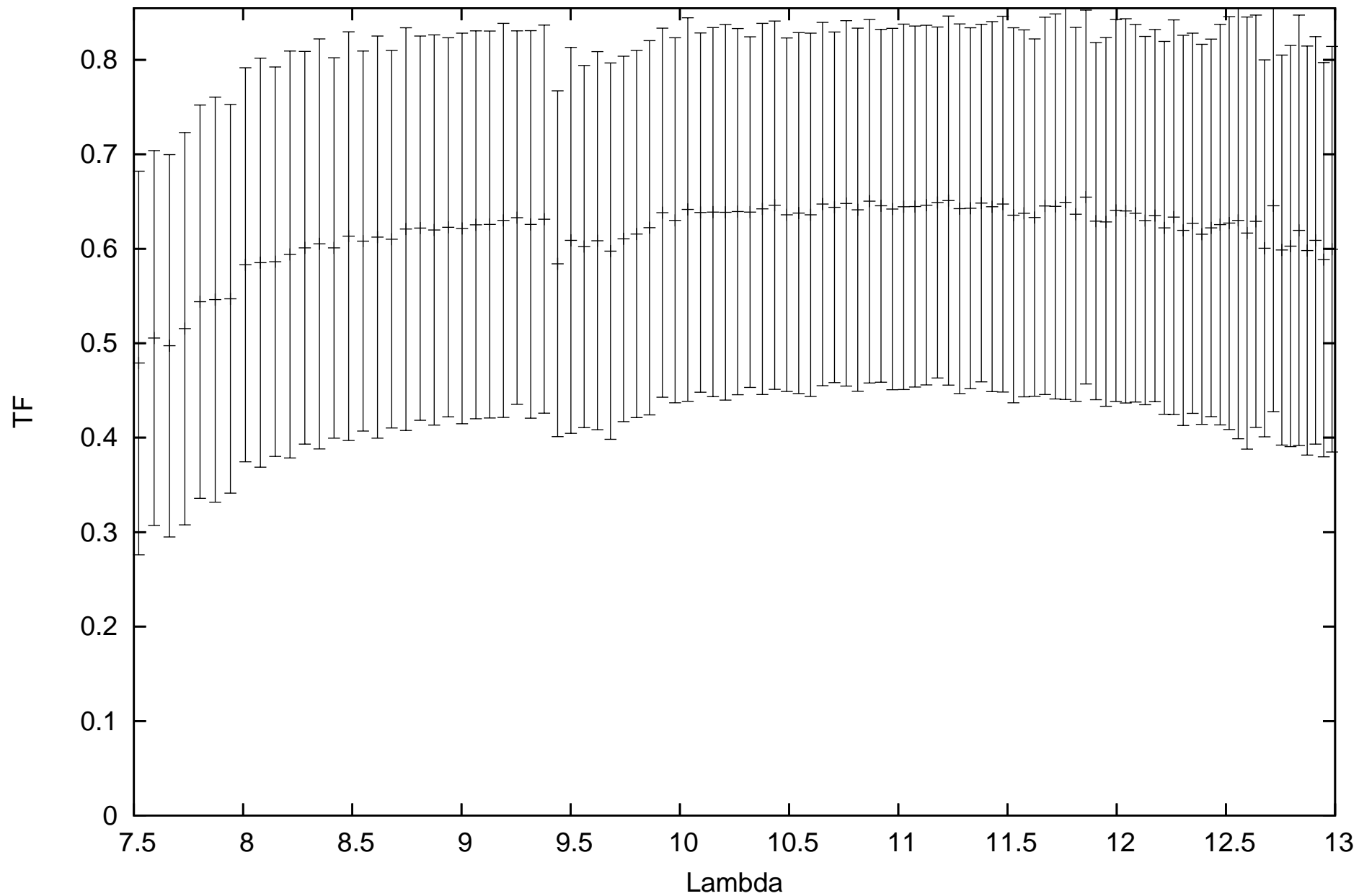
calHD081797_flux-1.49_diam9.14_r.MIDI.2010-04-13T03_27_47.000_D0H0
