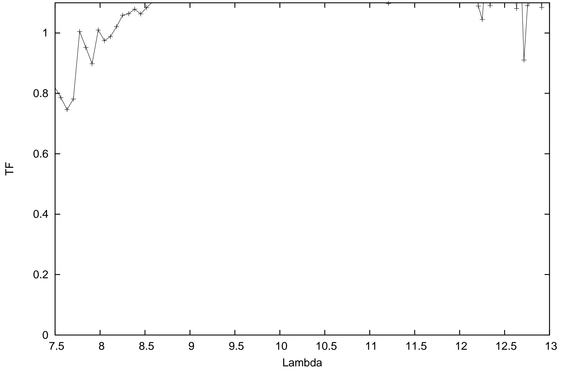
calHD081797_flux-1.49_diam9.14_r.MIDI.2010-04-13T03_02_11.138_D0G1
