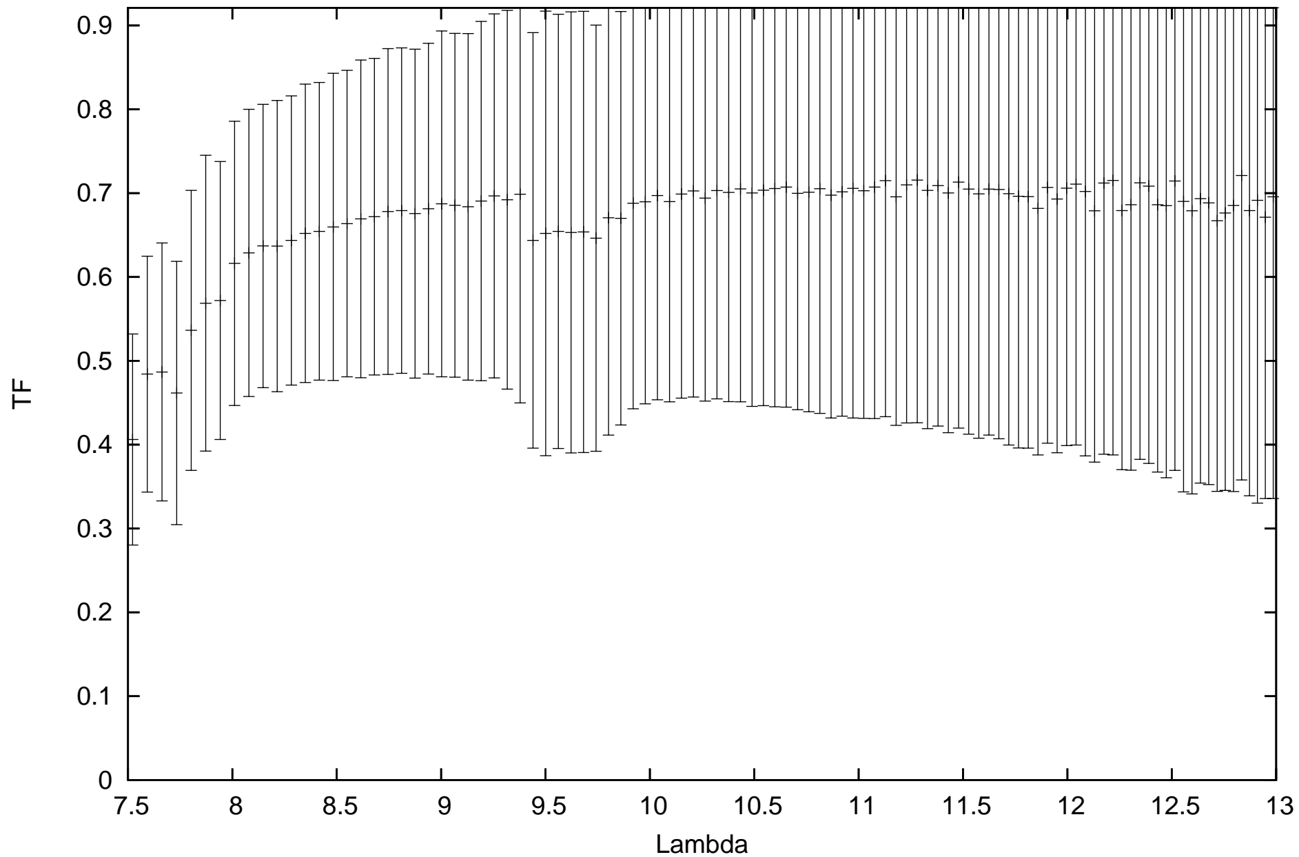
calHD126927_flux1.74_diam2.23_r.MIDI.2010-03-28T10_02_00.000_U1U4
