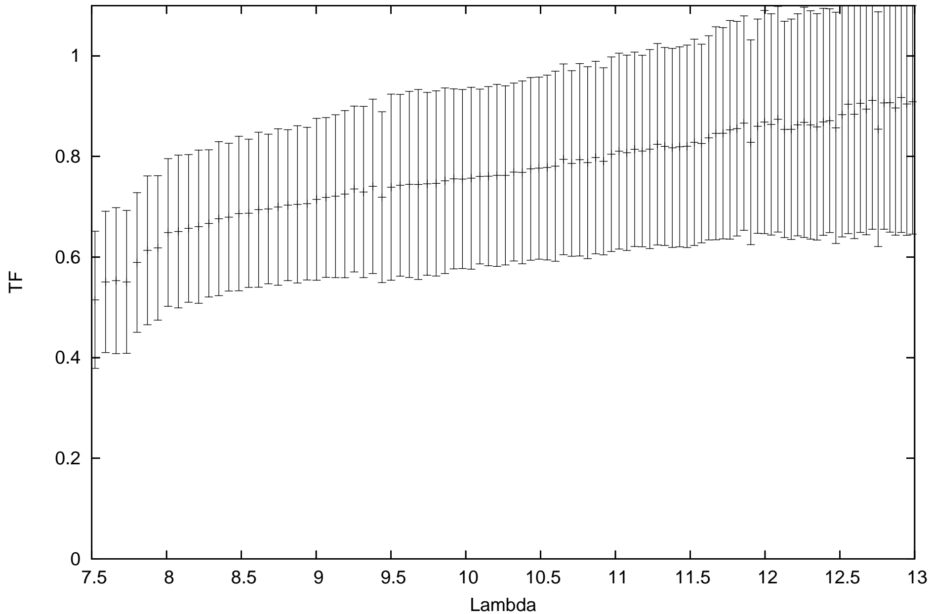
calHD123123_flux0.58_diam3.55_r.MIDI.2010-03-28T07_16_31.000_U1U4
