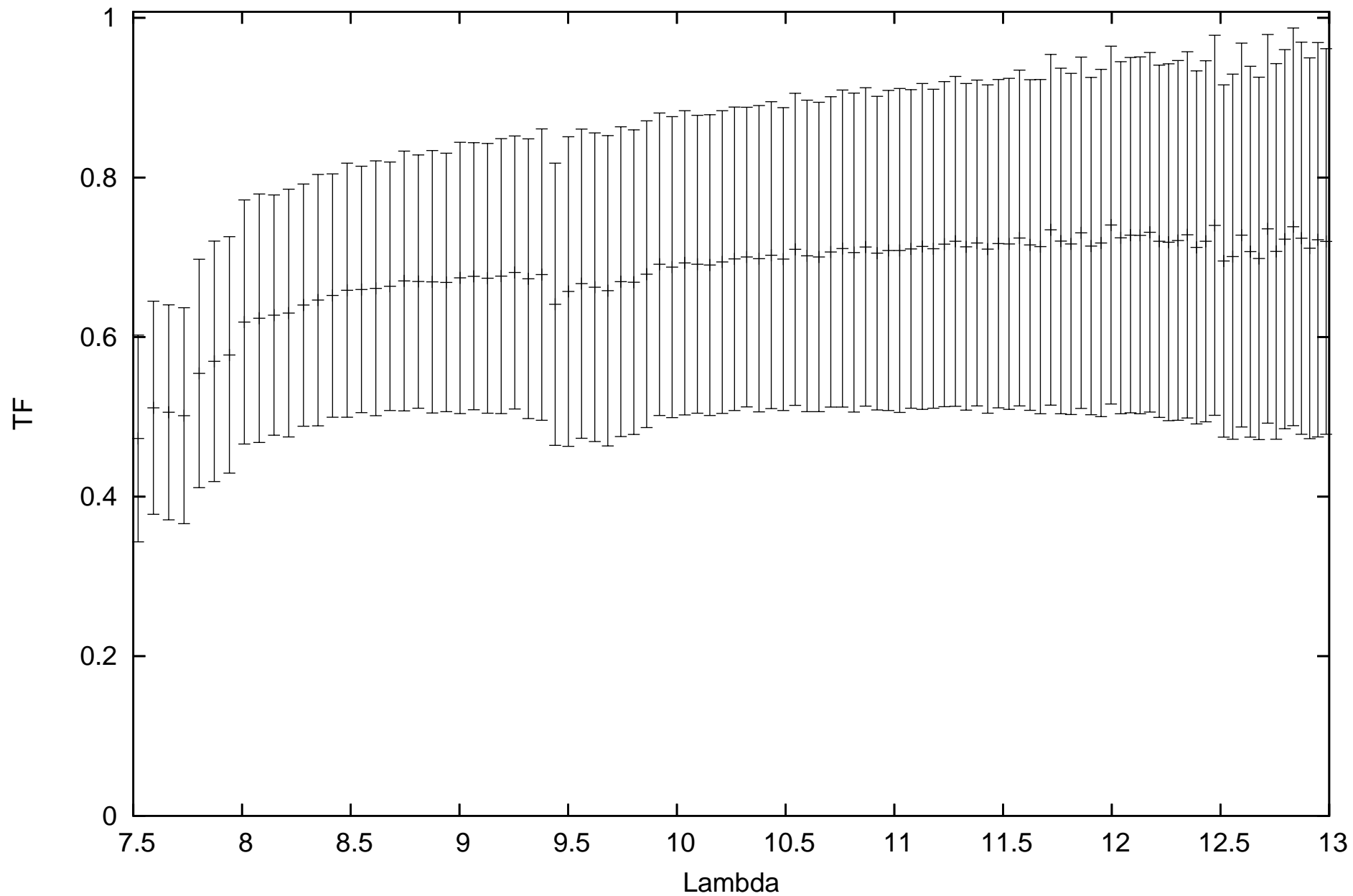
calHD090610_flux0.76_diam3.51_r.MIDI.2010-03-28T04_37_48.000_U1U4
