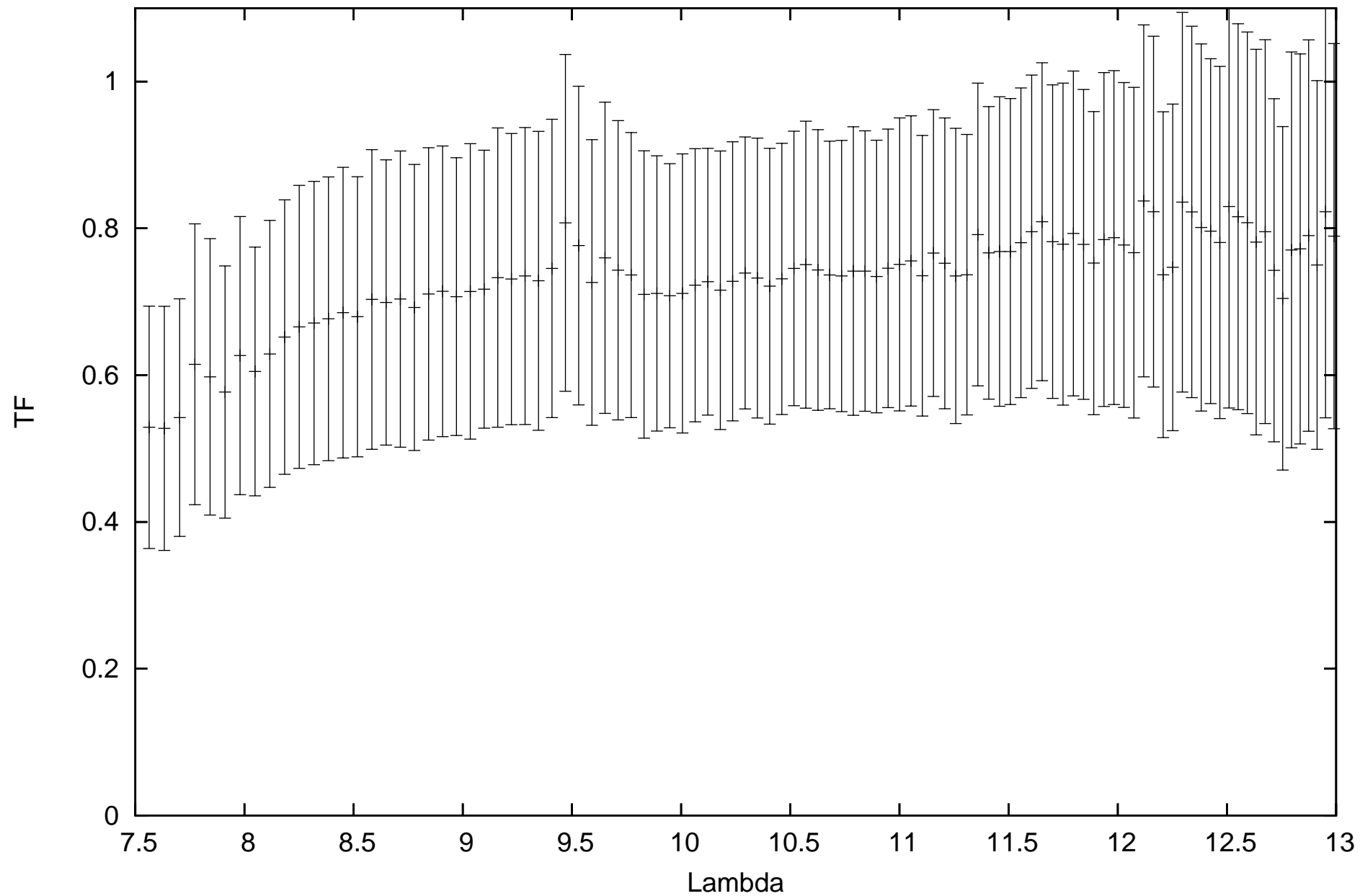
calHD120323_flux-2.02_diam13.25_r.MIDI.2010-03-21T06_47_39.015_H0G0
