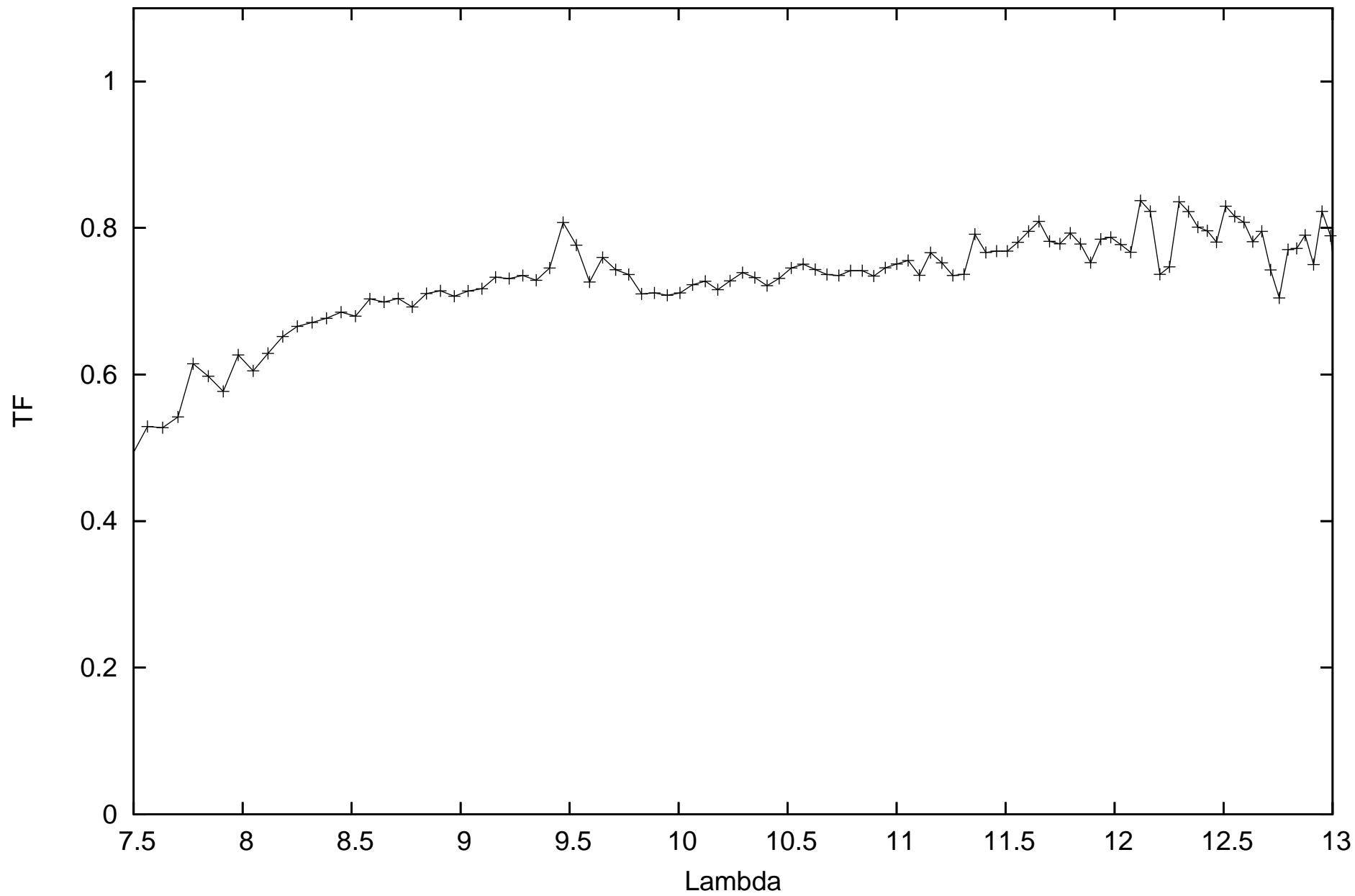
calHD120323_flux-2.02_diam13.25_r.MIDI.2010-03-21T06_47_39.015_H0G0
