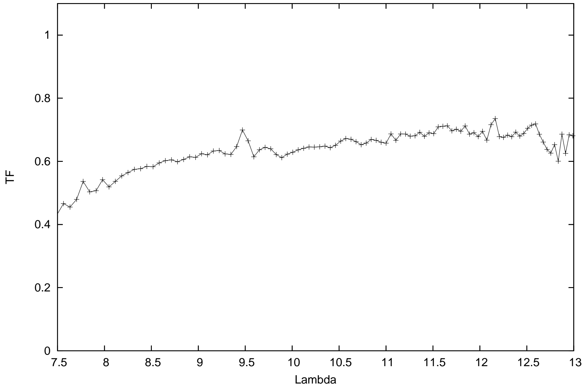
calHD120323_flux-2.02_diam13.25_r.MIDI.2010-03-16T09_02_02.850_H0D0
