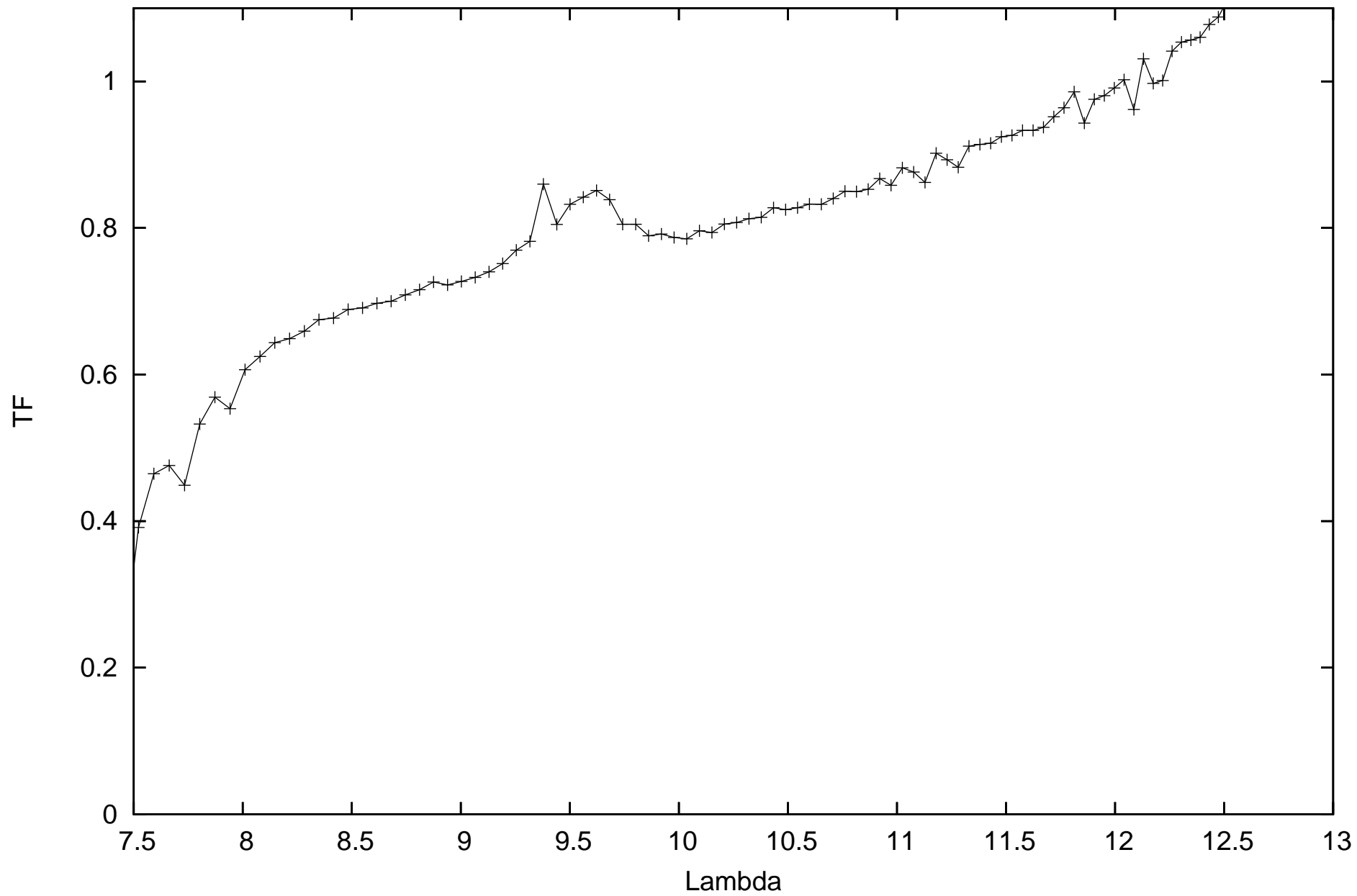
calHD031767_flux1.23_diam2.68_r.MIDI.2010-03-03T02_39_28.000_U3U4
