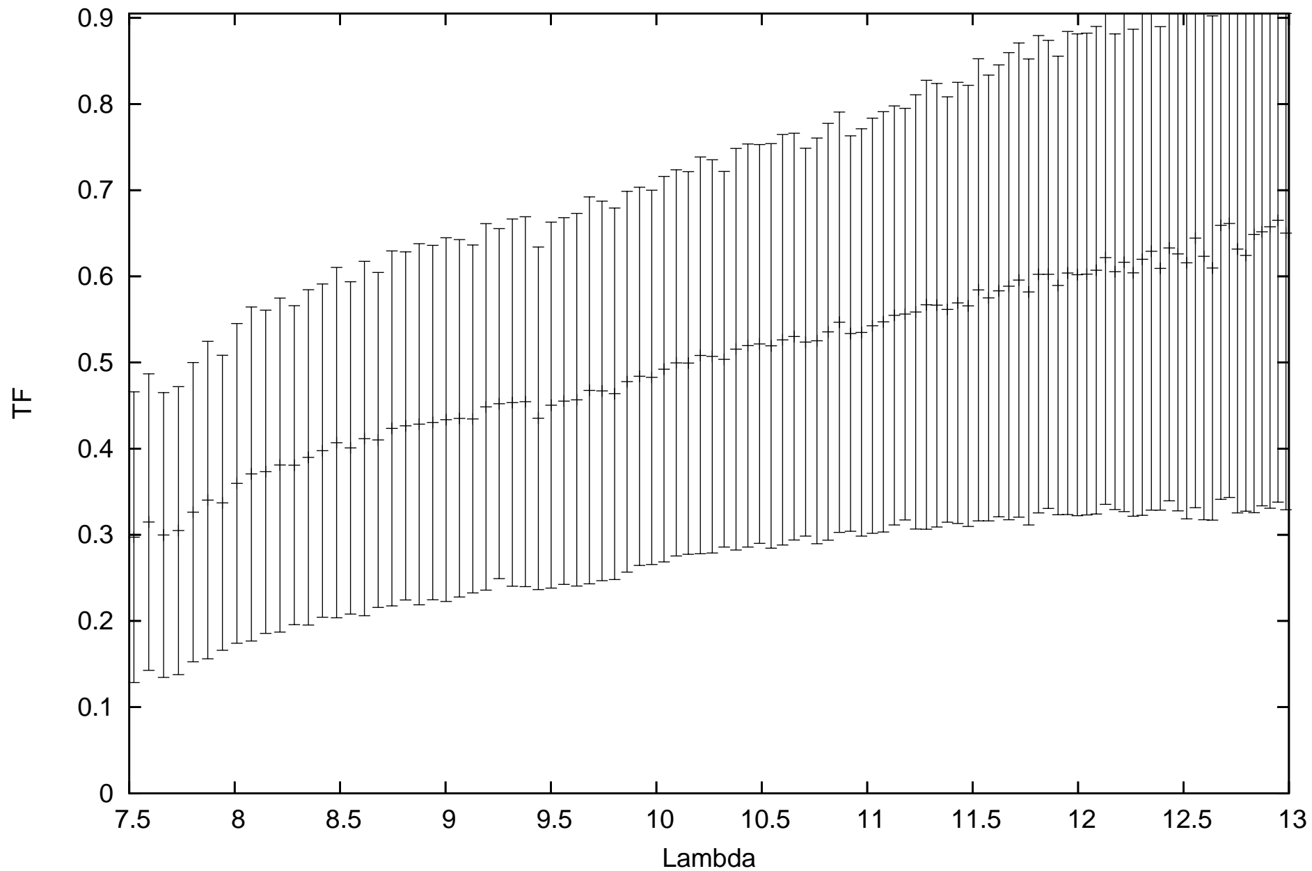
calHD112213_flux1.03_diam3.16_r.MIDI.2010-03-02T07_29_55.000_U1U3
