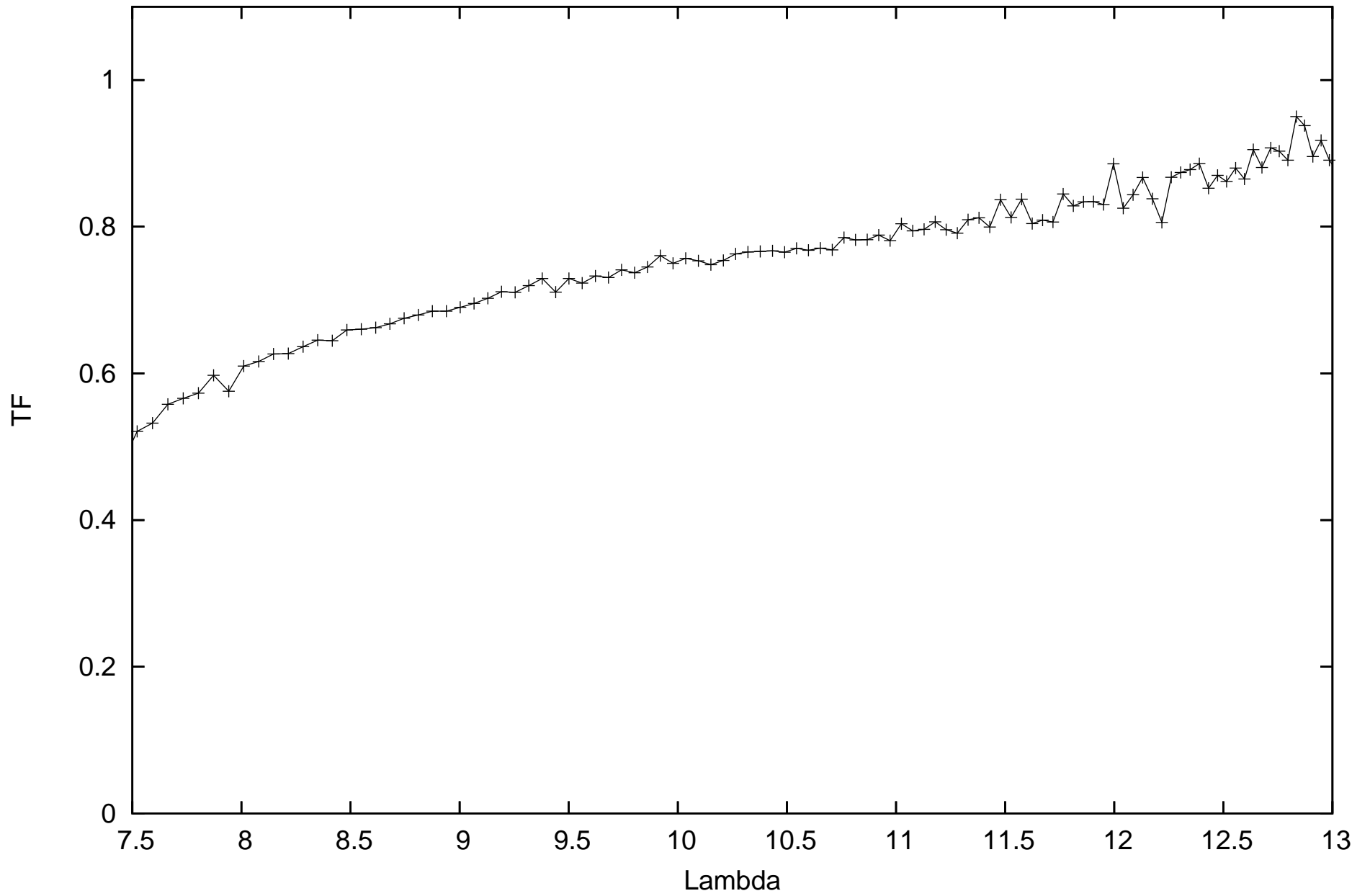
calHD081797_flux-1.49_diam9.14_r.MIDI.2010-02-25T04_11_17.000_DOKO
