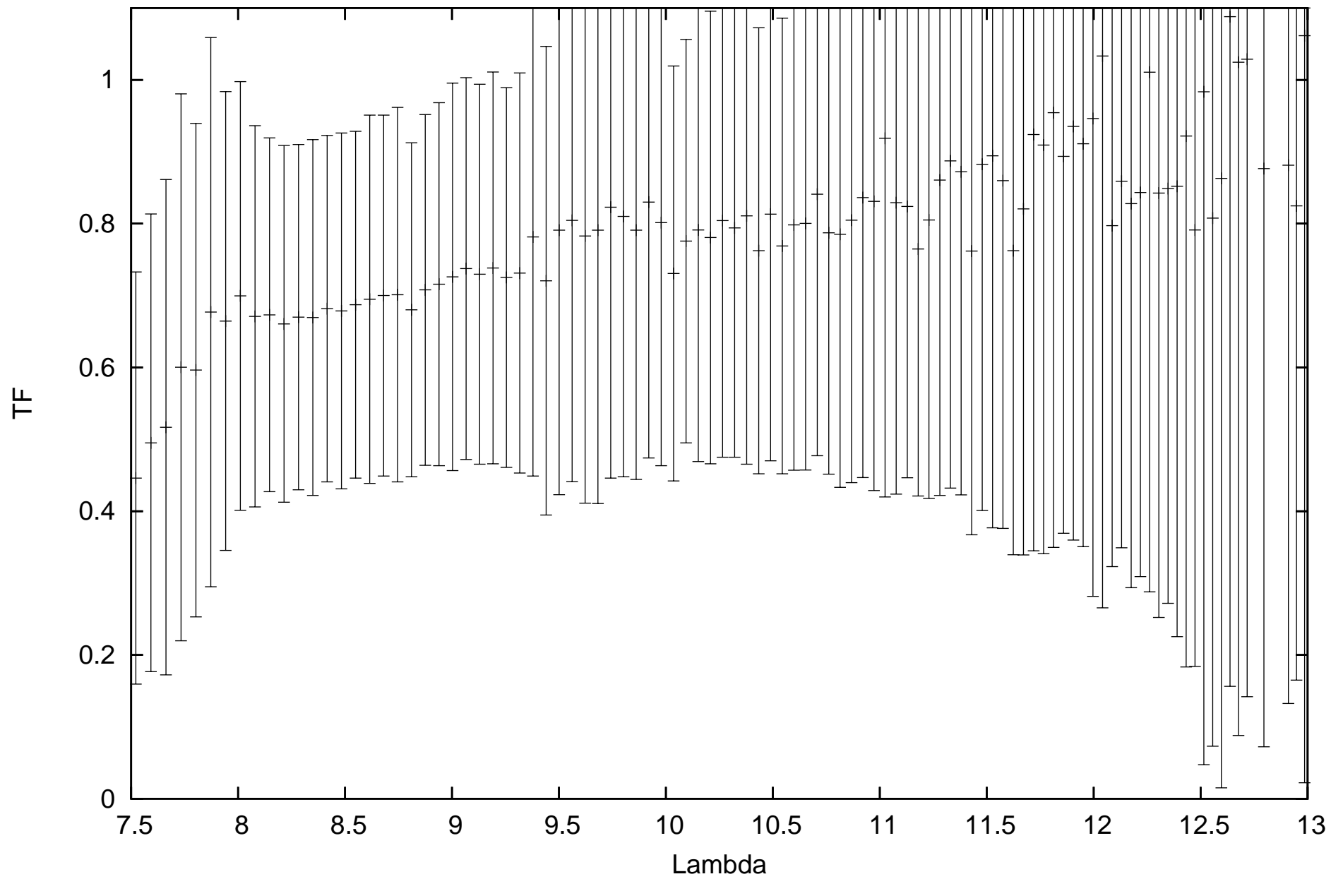
calHD054605_flux0.14_diam3.56_r.MIDI.2010-02-14T02_45_30.000_E0G0
