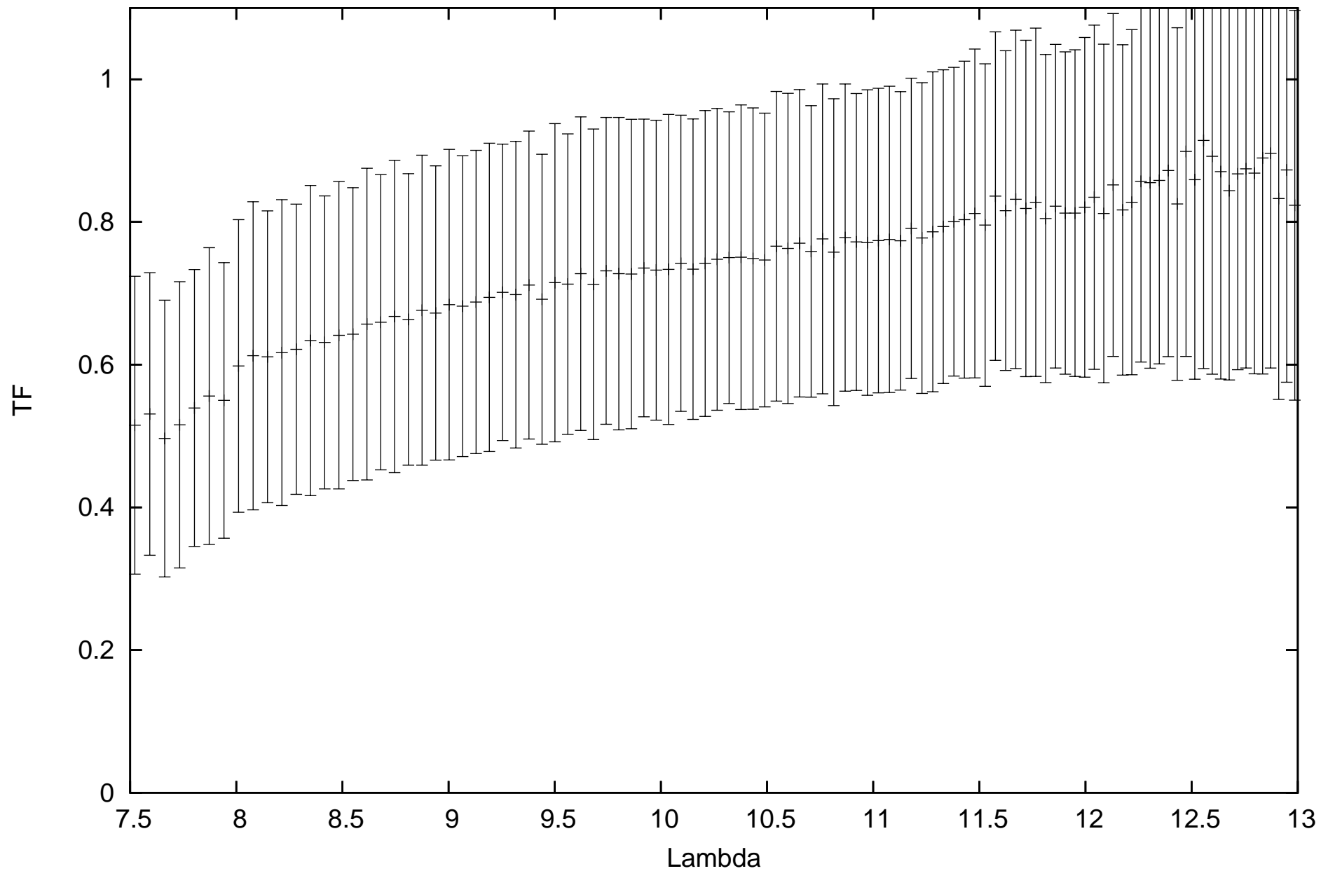
calHD048915_flux-1.39_diam6.09_r.MIDI.2010-02-14T03_08_46.000_E0G0
