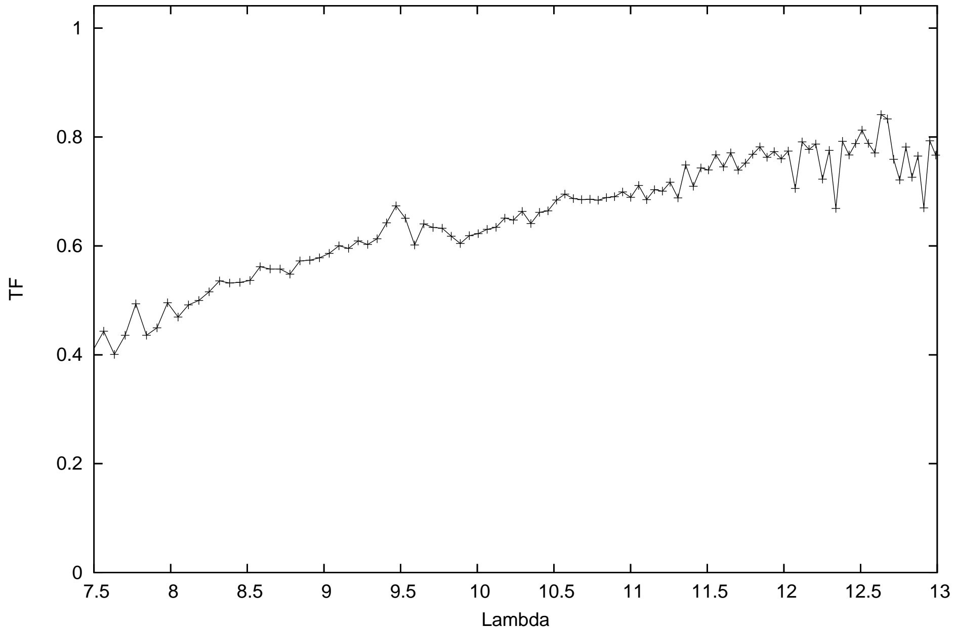
calHD048915_flux-1.39_diam6.09_r.MIDI.2010-02-14T02_17_23.644_E0G0
