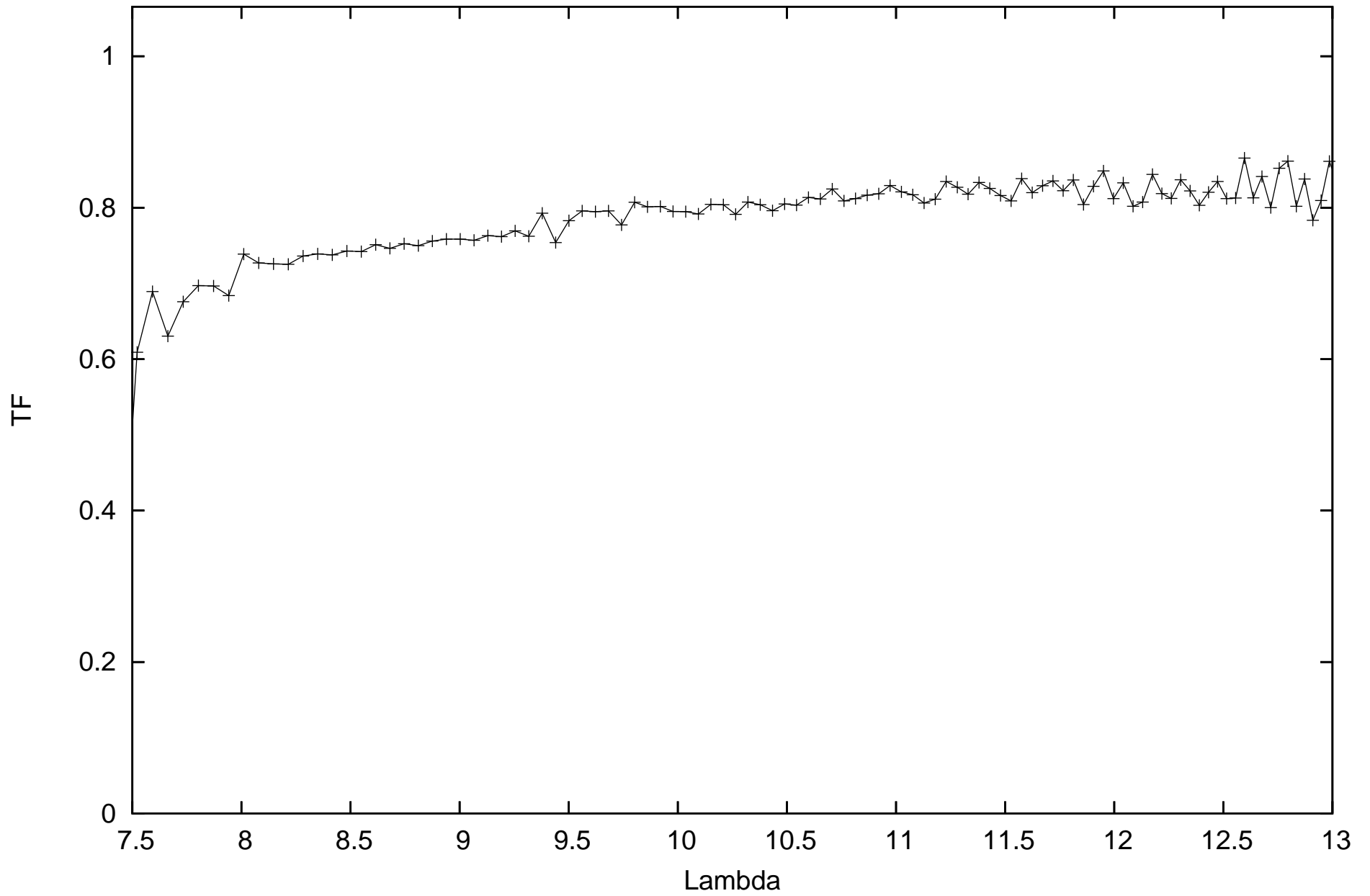
calHD045348_flux-1.47_diam6.87_r.MIDI.2010-02-13T04_33_54.000_H0G0
