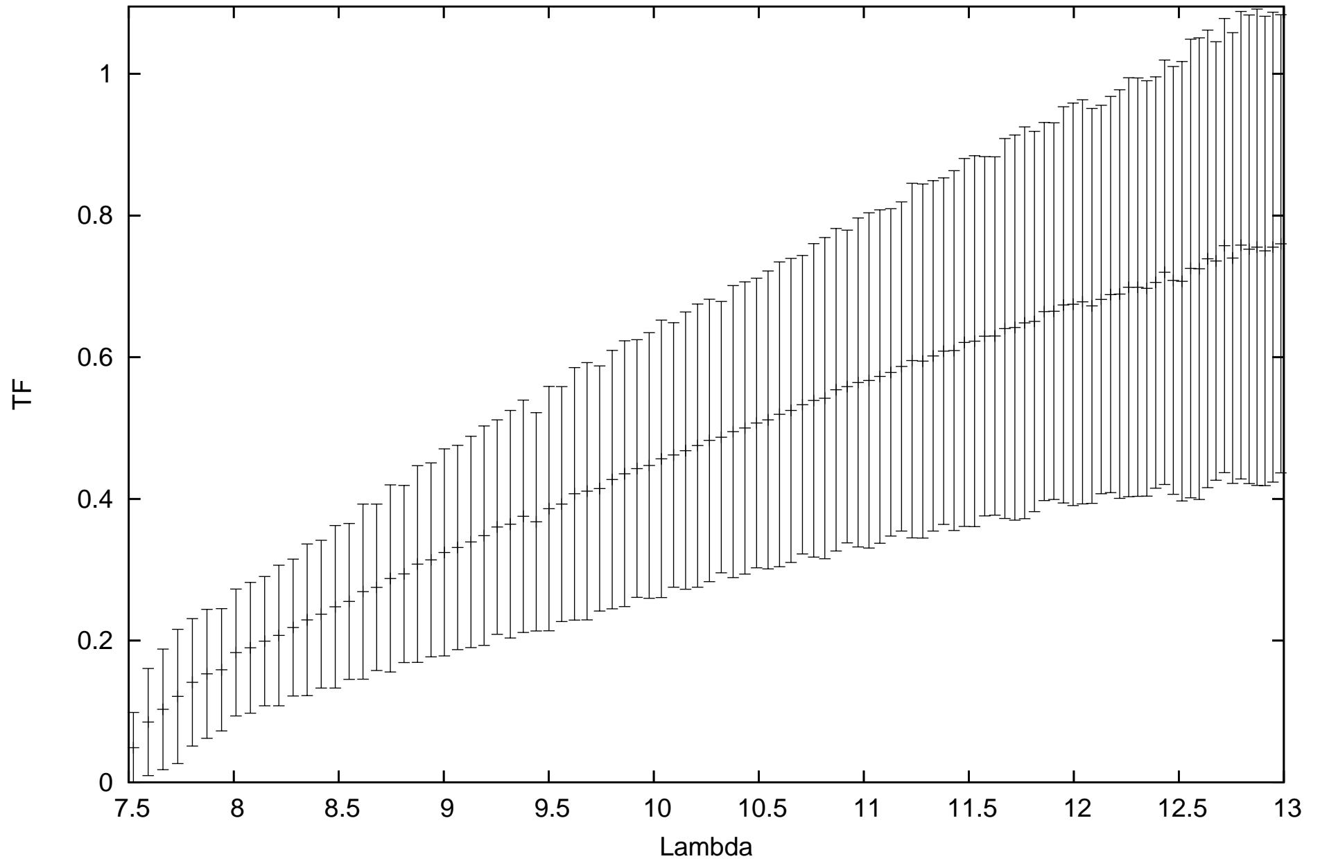
calHD029139_flux-3.11_diam20.4_r.MIDI.2010-02-13T00_21_11.000_K0E0
