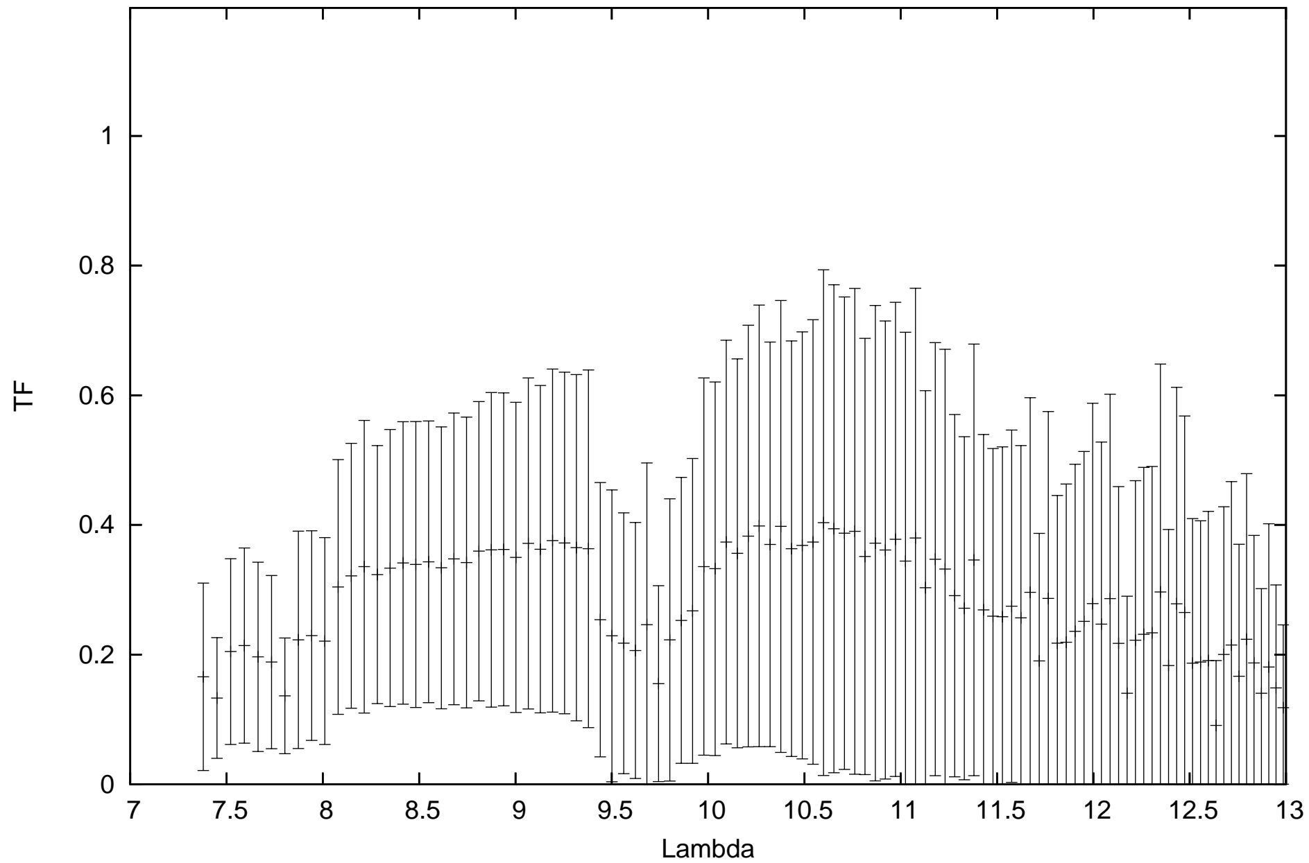
calhd169916_flux0.43_diam3.9_r.MIDI.2008-09-27T02_45_30.000_HIGHSENS
