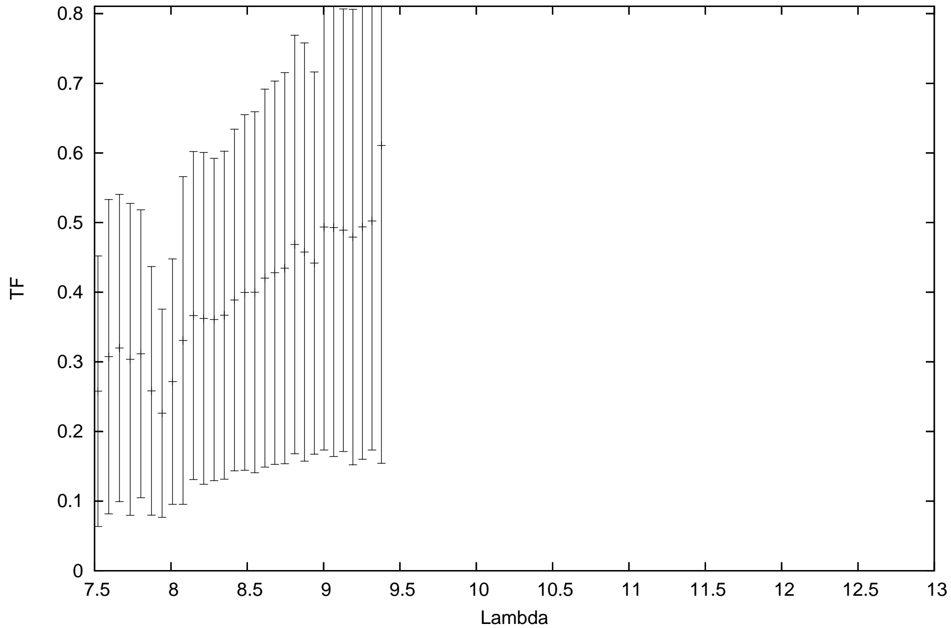
calhd169916_flux0.43_diam3.9_r.MIDI.2007-07-28T07_12_31.000_H0D0
