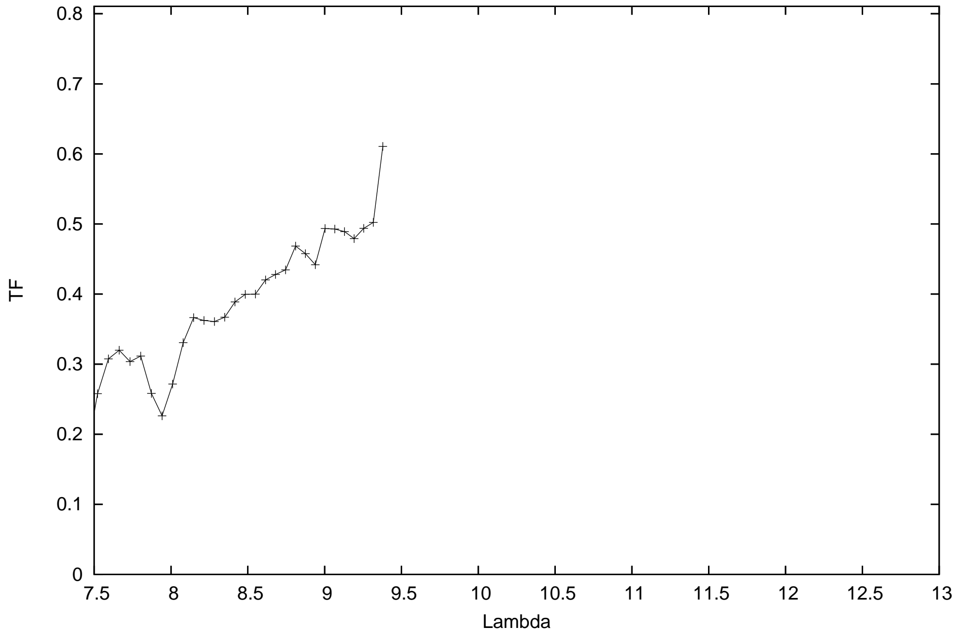
calhd169916_flux0.43_diam3.9_r.MIDI.2007-07-28T07_12_31.000_H0D0
