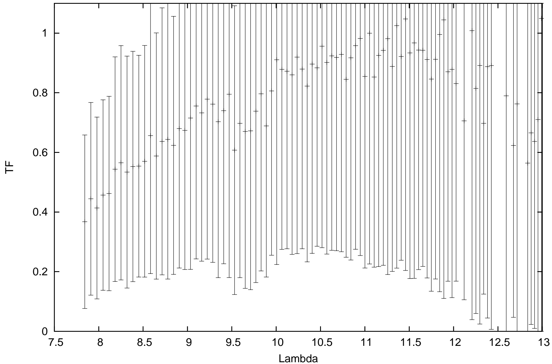
calHD224935_flux-0.85_diam7.24_r.MIDI.2009-10-21T04_30_05.686_H0D0
