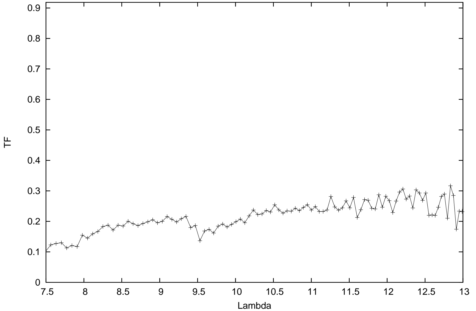
calHD224935_flux-0.85_diam7.24_r.MIDI.2009-10-02T05_32_46.687_E0H0
