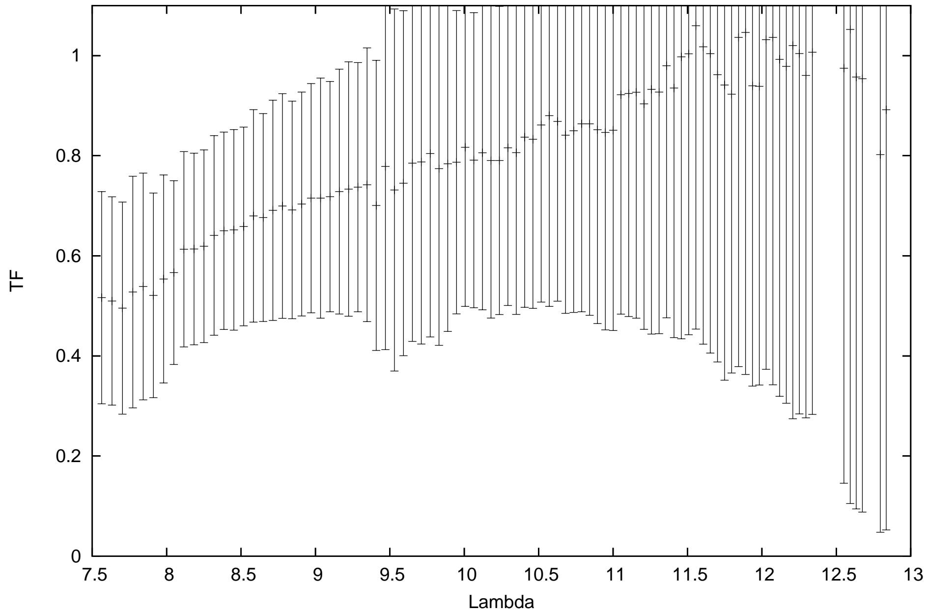
calHD224935_flux-0.85_diam7.24_r.MIDI.2009-08-14T09_07_14.686 SCIPHOT
