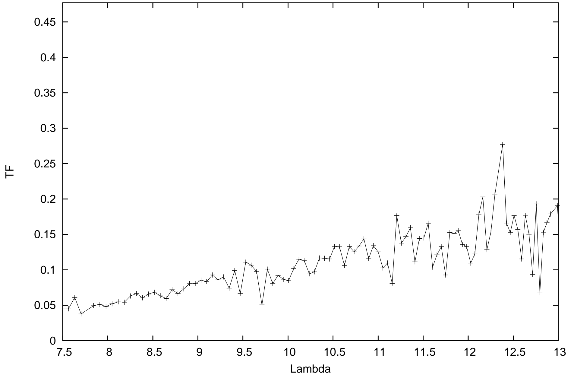
calHD224935_flux-0.85_diam7.24_r.MIDI.2009-08-14T07_49_49.687 SCIPHOT
