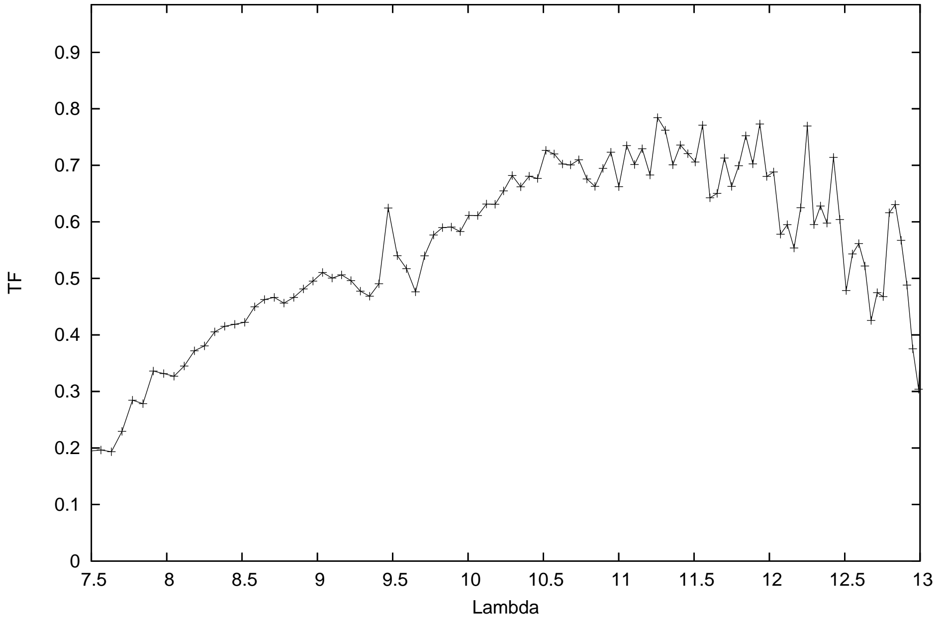
calHD224935_flux-0.85_diam7.24_r.MIDI.2009-07-30T08_27_47.029 SCIPHOT
