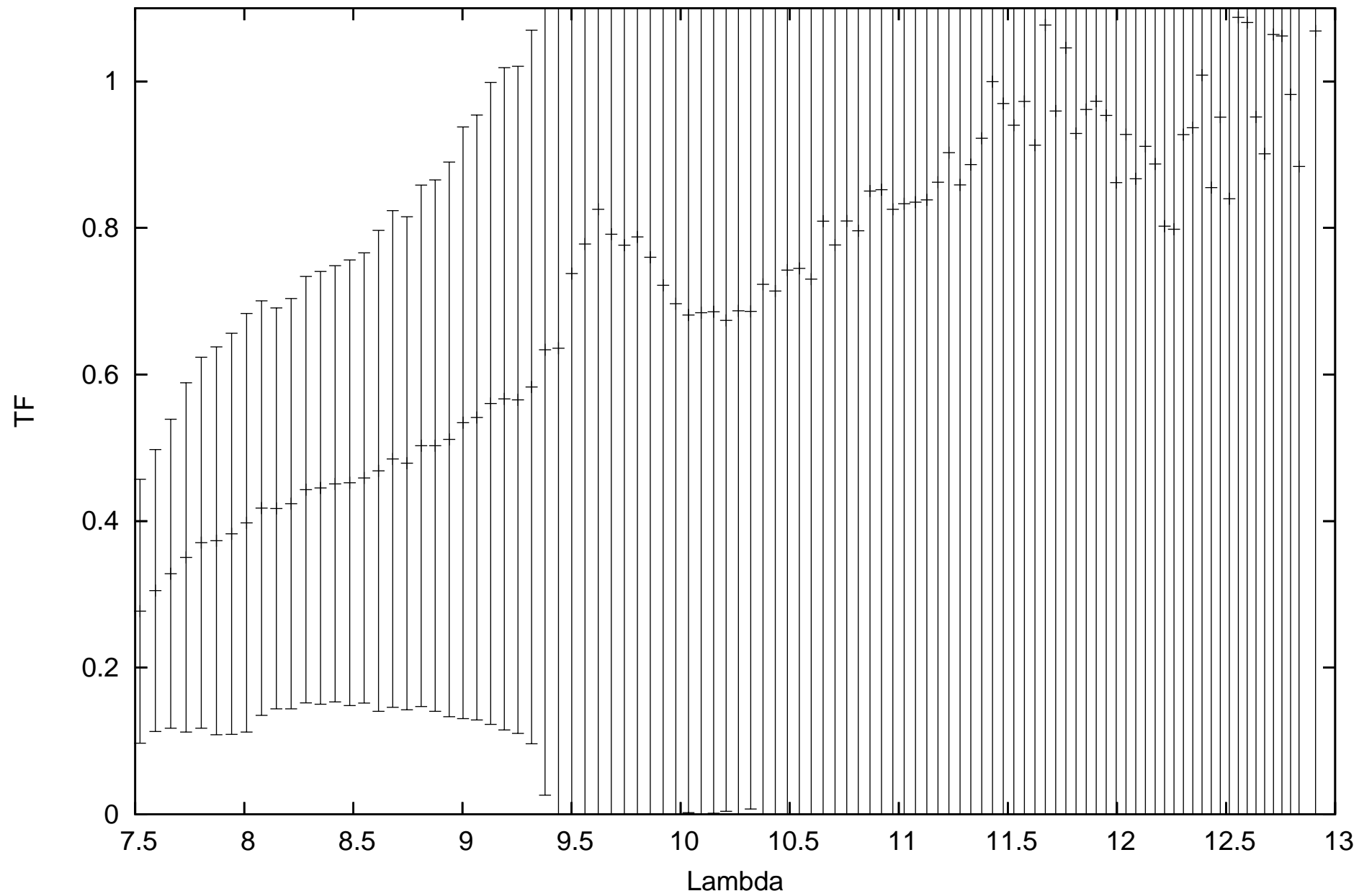
calHD224935_flux-0.85_diam7.24_r.MIDI.2008-09-27T05_18_53.000_HIGHSENS
