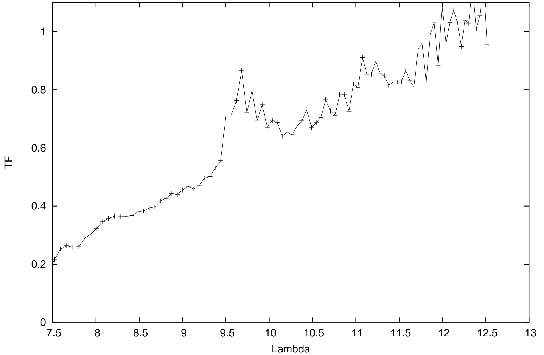
calHD216386_flux-0.89_diam7.58_r.MIDI.2008-09-27T04_12_55.000_HIGHSENS
