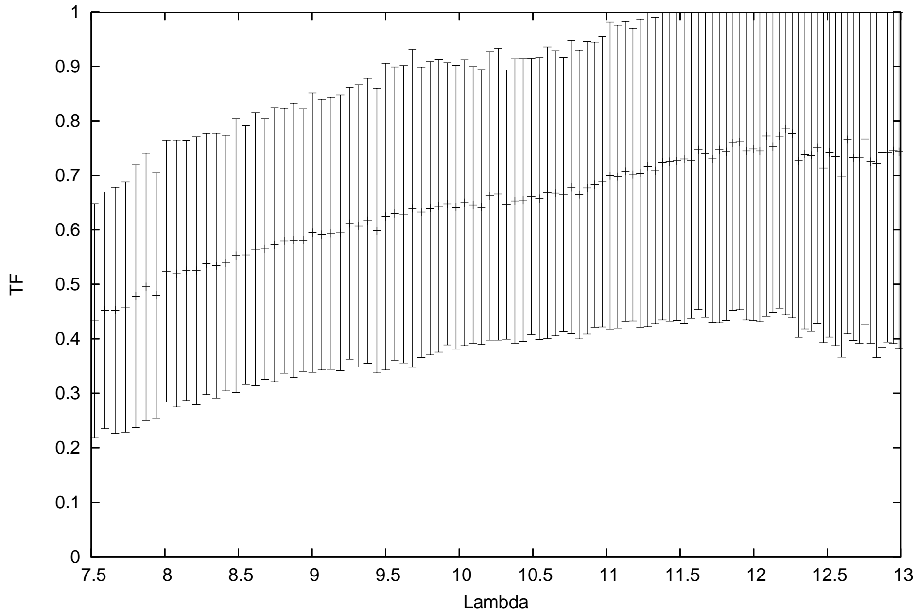
calHD206778_flux-1.04_diam7.59_r.MIDI.2009-11-15T01_24_23.000_E0G0
