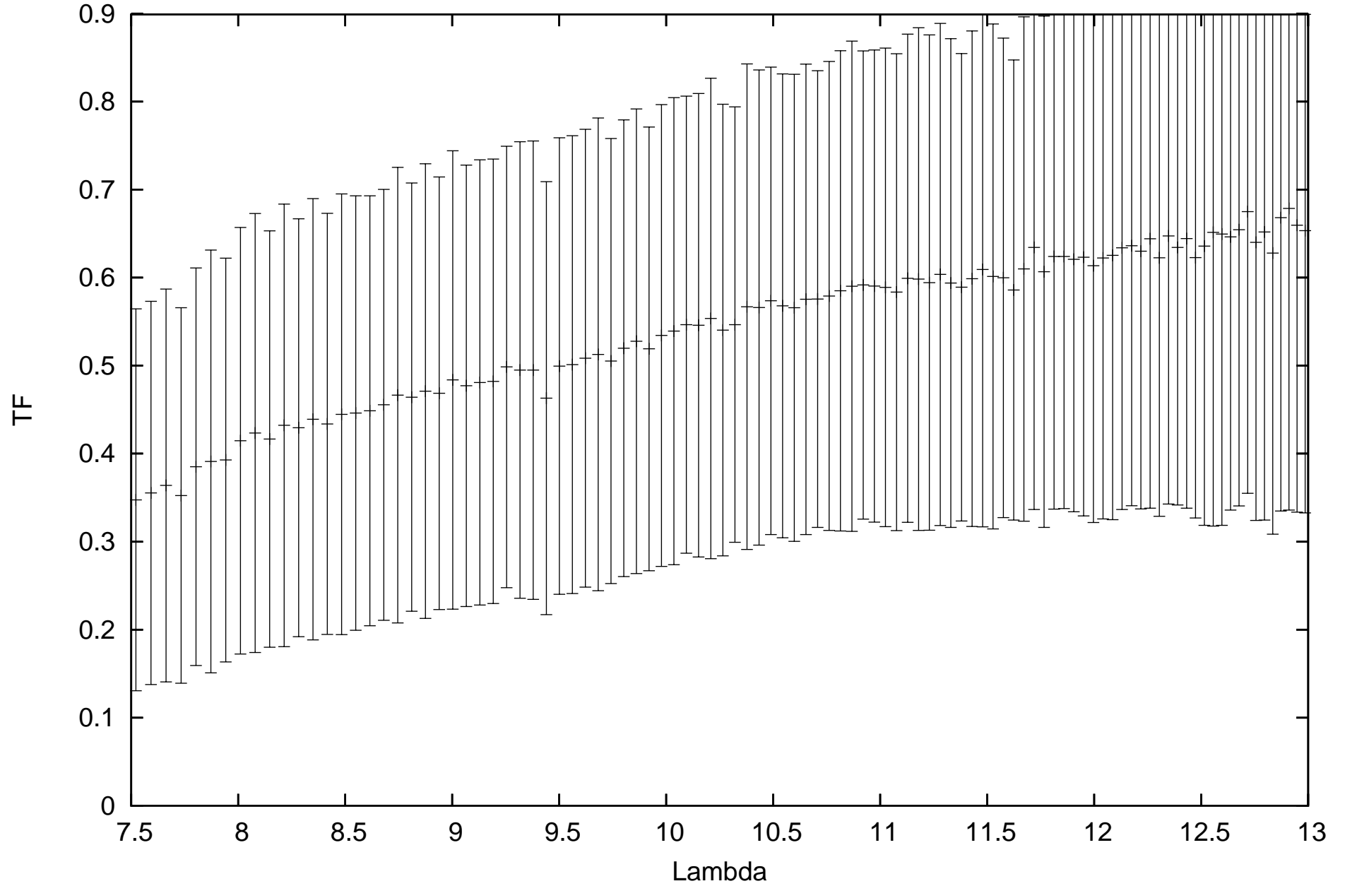
calHD206778_flux-1.04_diam7.59_r.MIDI.2009-10-01T03_12_26.000_HIGHSENS
