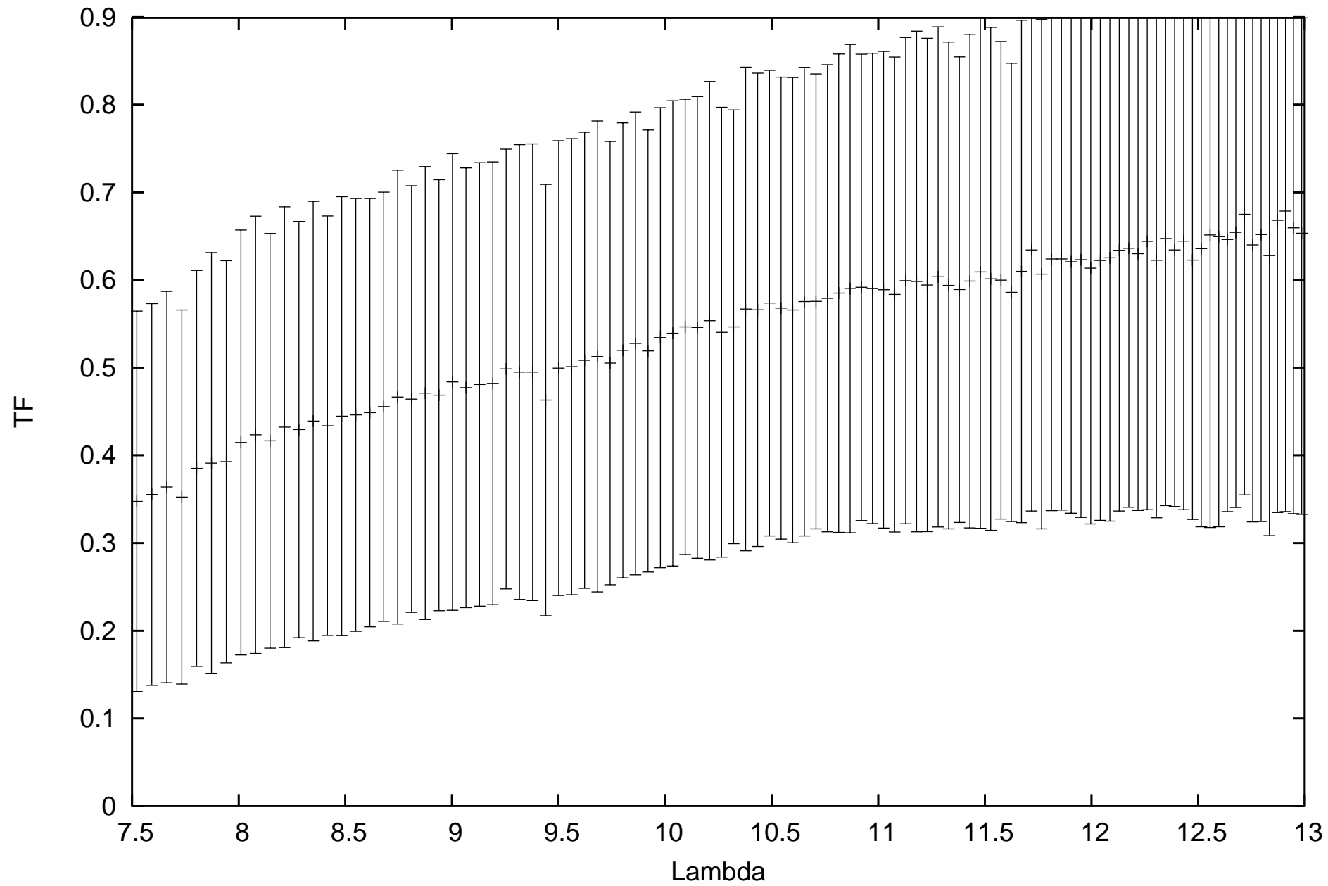
calHD206778_flux-1.04_diam7.59_r.MIDI.2009-10-01T03_12_26.000_E0H0
